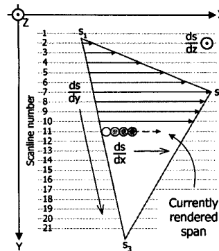
Figure 3: Interpolations when drawing a triangle on the screen.
