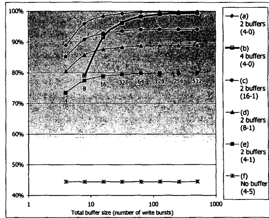
Figure 7: Memory bandwidth utilization as a function of buffer size. The input data is assumed totally randomized. The numbers in parentheses refer to (Write Cycles – Wait Cycles).
