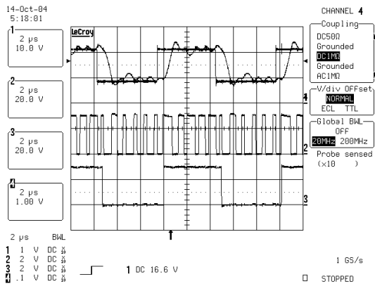
Figure 12 Output and reference voltages (top), HF (middle) and LF (bottom) buck PWM output voltages. Converter driving 100kHz 12\text{Vpp}+15\text{VDC} square into 8\Omega .
