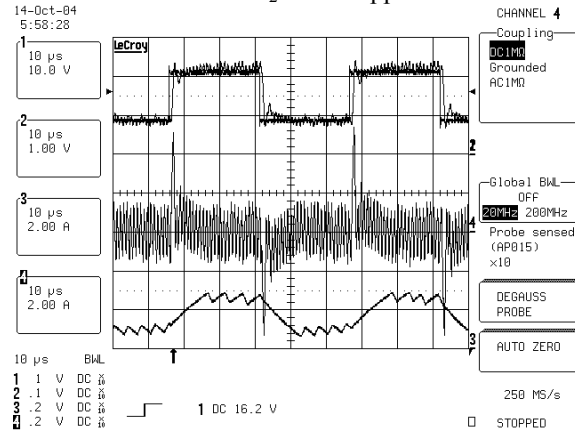
Figure 15 Output and reference voltages (top), HF (middle) and LF (bottom) buck inductor current. Converter driving 20kHz 12\text{Vpp}+15\text{VDC} square into 8\Omega .
