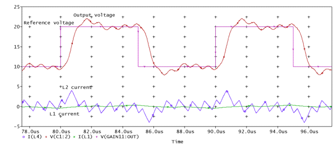
Figure 10 Simulated output (red) and reference voltages (magenta), L_2 (blue) and L_1 (green) buck inductor current. Converter driving 100kHz 10Vpp+15VDC square wave response into open load.
