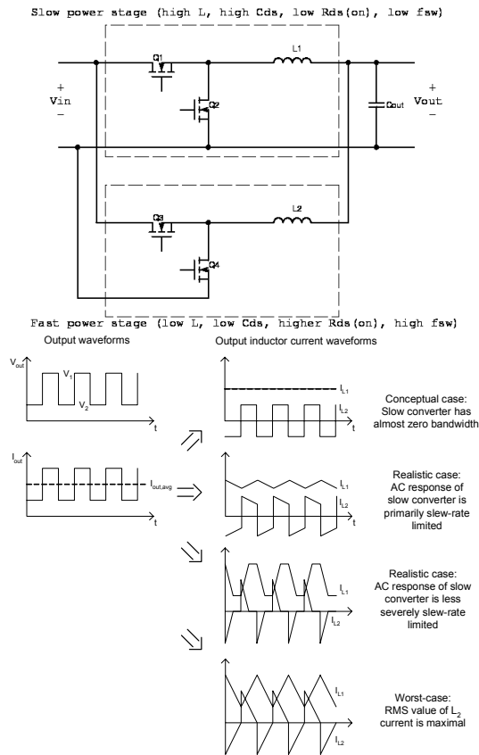
Figure 2 Principal illustration of the proposed power conversion scheme.
