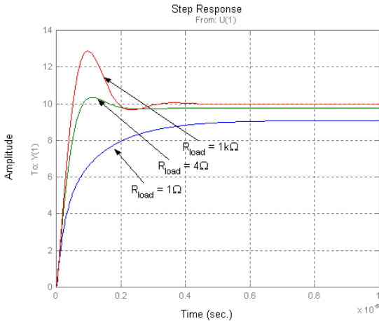
Figure 8 Step responses of closed voltage control loop showing that fast and well damped responses are achievable using the proposed control scheme.
