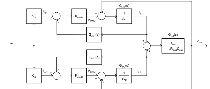
Figure 3 Block diagram of paralleled, current controlled buck converters.
