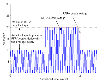
Figure 1 Idealized example of envelope tracking supply voltage for an RFA for 16-QAM signal amplification.
