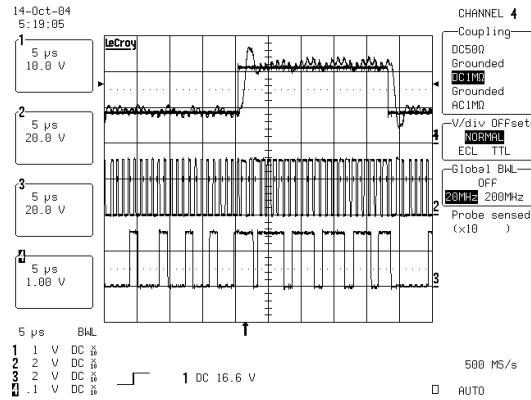
Figure 14 Output and reference voltages (top), HF (middle) and LF (bottom) buck PWM output voltages. Converter driving 20kHz 12\text{Vpp}+15\text{VDC} square into open load.
