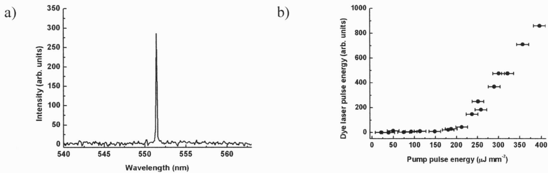
Fig. 2. a) Emission spectrum from the dye laser when pumped with 5 ns pulses at a pump energy density of 396 μJ/mm 2 . The linewidth reflects the limited resolution of the spectrometer (0.15 nm). b) Dye laser output as function of pump energy, the lasing threshold is observed at 210 μJ/mm 2 . The horizontal error bars on the pump energy is due to pump laser fluctuations. The error on the vertical axis is smaller than the size of the dots.
