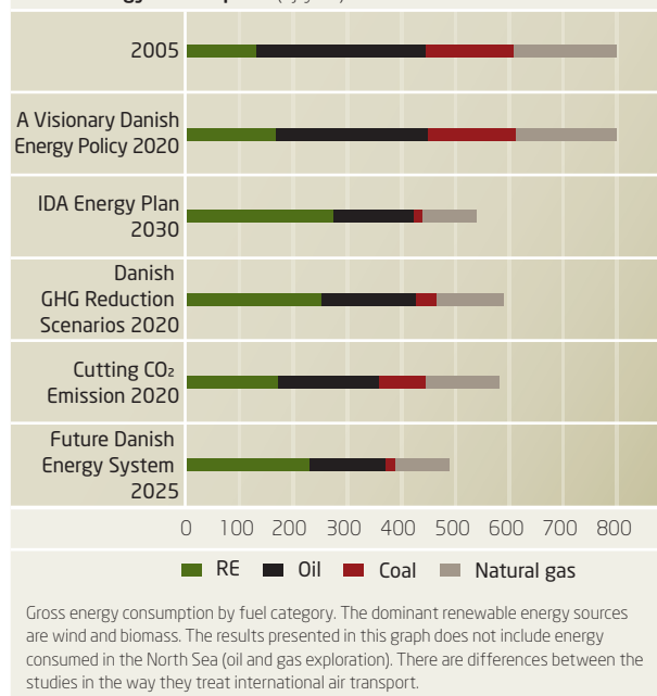
Figure 25 Gross energy consumption (PJ/year)
