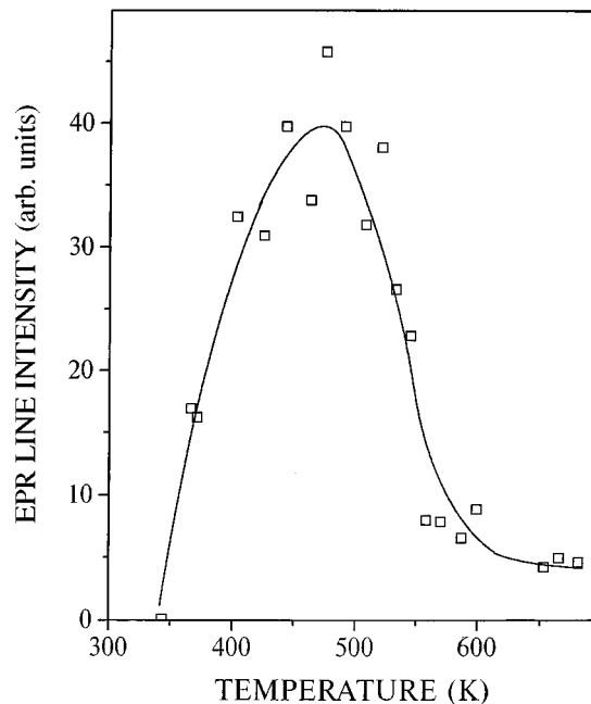
FIG. 2. Temperature dependencies of the EPR signal intensity in Gd-containing LB film (sample A) during heating. Solid lines are guides for the eye.
