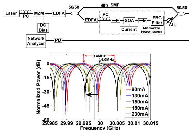
Fig. 2. Experimental set-up of a two-arm microwave photonic notch filter (upper) and measured filter response (lower) [14]. Notice that the path difference between the two arms is chosen long enough that the optical fields from the two arms combine incoherently . The RF response of the microwave photonic notch filter obtained by changing the injection current of the SOA is shown for the modulator biased at a voltage of 4.5 V. A similar but opposite shift of the filter response is obtained when the modulator voltage is set at 8.1 V. The dotted lines are simulation results based on a simple four-wave mixing model.
