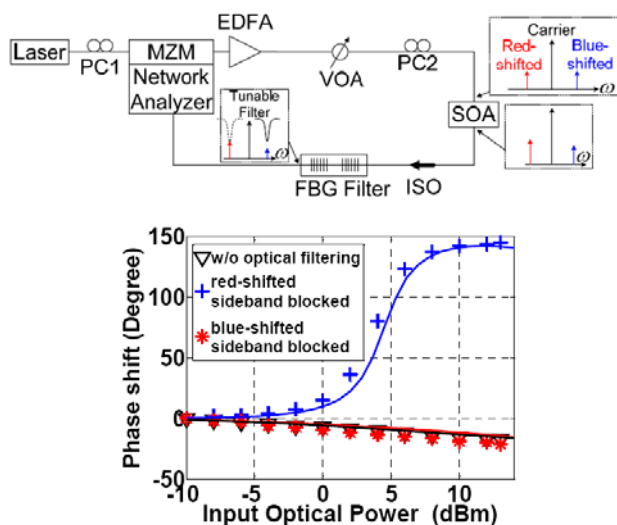
Fig. 1. Experimental set-up (upper) and results (lower) for the case of performing optical filtering before detection [12]. A fiber-grating (FBG) notch filter allows one of the sidebands to be blocked before detection without influencing the carrier or the other sideband. The modulation frequency is 19 GHz. Markers are experimental data and solid lines are numerical simulations. Three cases are shown: no filtering (black); blocking the blue-sideband and letting the red pass (red); blocking the red sideband and letting the blue pass (blue). The simulations were performed using a four-wave mixing model for the interaction of the different sideband, taking into account only the dynamics of the total carrier density.
