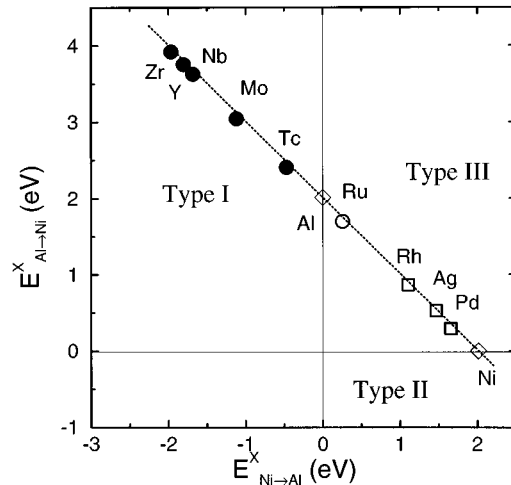
FIG. 3. The energies of moving ternary additions from \text{Ni} to \text{Al} sites E_{\text{Al} \rightarrow \text{Ni}}^X and from \text{Al} to \text{Ni} sites E_{\text{Ni} \rightarrow \text{Al}}^X defined at the point (1,1) of the LRO space on the basis of the ordering energies (14) of \text{Ni}_{70.5}\text{Al}_{23.5}\text{X}_6 ternary alloys. The line E_{\text{Al} \rightarrow \text{Ni}}^X + E_{\text{Ni} \rightarrow \text{Al}}^X = E_{\text{ant}}^{\text{xc}} where E_{\text{ant}}^{\text{xc}} = 2.0 eV is the energy of antisite defect formation of the completely ordered \text{Ni}_3\text{Al} . The filled circles are the additions with a strong preference (sufficient to create antisite defects) for occupation of \text{Al} sites (type I), open circles are the additions with a weak preference (insufficient to create antisite defects) for \text{Al} sites [type III ( \text{Al} )] and open squares are the additions with a weak (insufficient to create antisite defects) preference for \text{Ni} sites. The open diamonds correspond to the substitution behavior of \text{Al} and \text{Ni} atoms as ternary additions.
