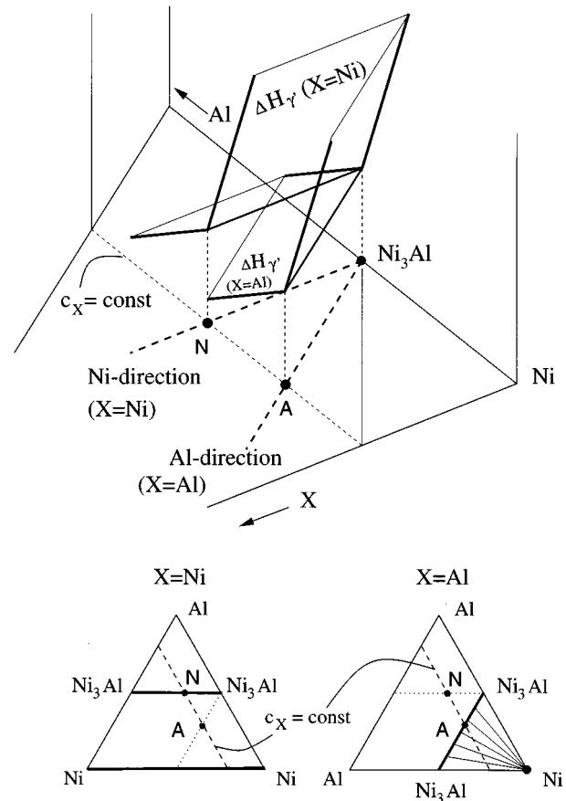
FIG. 14. Schematic presentation of the surfaces of the enthalpies of formation of the \gamma' phase in the coordinates of the triangle of ternary alloy compositions for X = \text{Ni} and Al. Bold lines correspond to the section of these surfaces by the planes \bar{c}_X = 0 and \bar{c}_X = \text{const} . The points N and A indicate the position of the fold on the line \bar{c}_X = \text{const} . The corresponding phase diagrams at 0 K for Ni-Al-Ni and Ni-Al-Al systems are shown in the lower part of the figure. Bold lines corresponds to \text{Ni}_3\text{Al} and pure Ni. Thin lines in the Ni-Al-Al phase diagram show tie-lines which in this particular case are generated only by one common-tangent plane. For the Ni-Al-Ni system any line connecting points of the \text{Ni}_3\text{Al} and Ni phases is the tie-line. The region between the "Ni-direction" and the "Al-direction" constitutes the region of quasistoichiometric alloy compositions.
