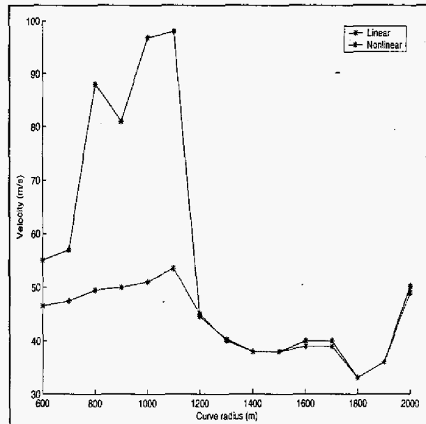
Figure 3. THE CRITICAL SPEEDS FOUND BY PETERSEN AND HOFFMANN [6]. THE SUPERELEVATION IS 2^\circ . NEAR R=1200\text{m} A SUBCRITICAL HOPF BIFURCATION SUDDENLY CHANGES TO A SUPERCRITICAL HOPF BIFURCATION
