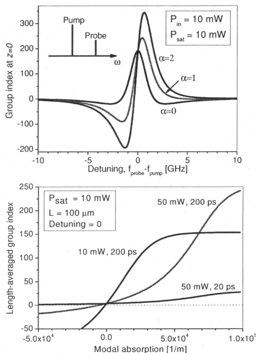
Fig. 1. Calculated variation of group index with detuning (top; at waveguide input for an absorption coefficient of 5 \cdot 10^4 \text{ m}^{-1} ) and modal absorption (bottom; averaged over waveguide length).
