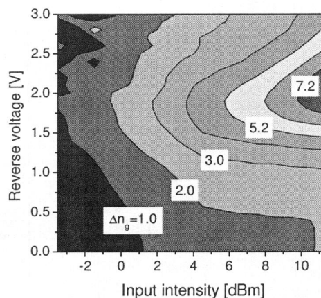
Fig. 2. Contour plot of measured change in group index versus input intensity and reverse voltage for a 100 \mu\text{m} long semiconductor waveguide.
