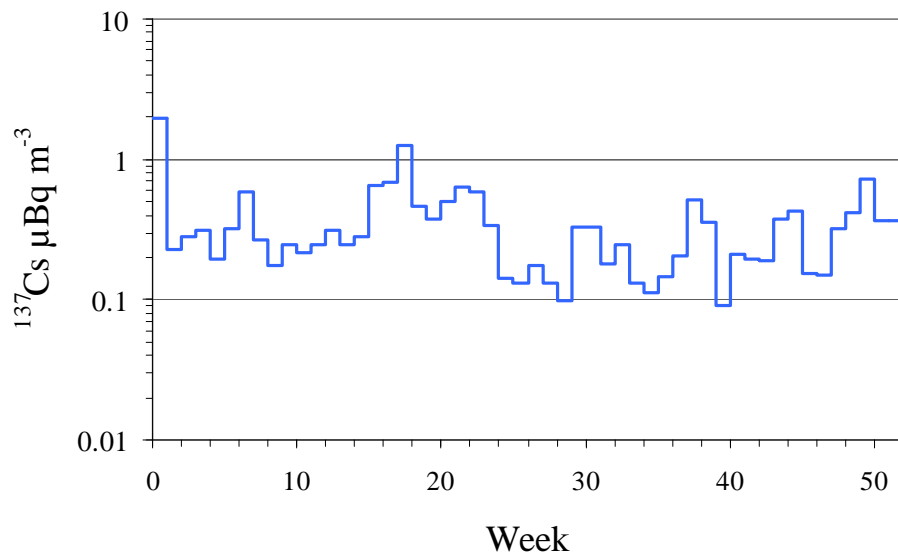
Fig. 1.1. Caesium-137 in ground level air collected at Risø in January-December 2008. (Unit: \mu\text{Bq m}^{-3} )
