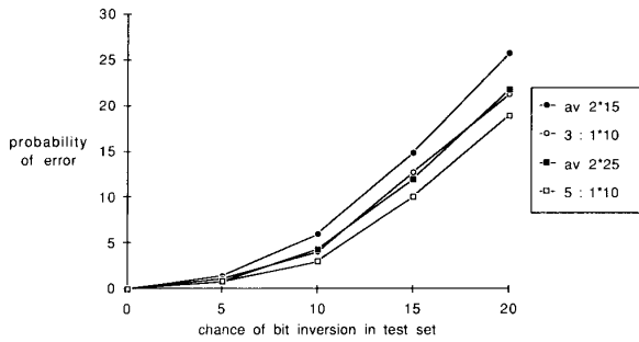
Fig. 6. The figure compares hidden neuron effectiveness as part of a second layer or as part of another network used in the ensemble. Performance curves are shown for ensembles of 3 and 5 single layer nets with 10 hidden neurons each which are to be compared with the average performance of nets with 15 and 25 neurons in each of two hidden layers. Note that the ensembles outperform the corresponding two layer nets.
