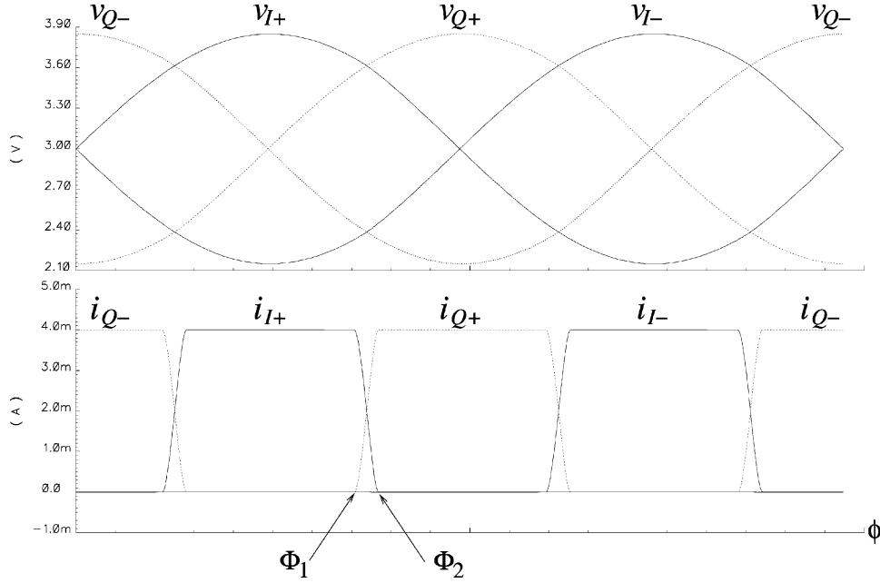
Fig. 5. Voltage and current waveforms for the I -half of the csPQO in Fig. 2.
