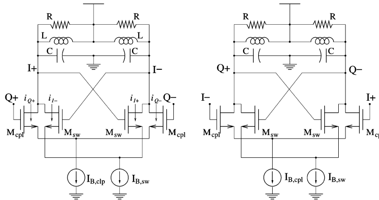
Fig. 1. Simplified schematic view of the dsPQO.
