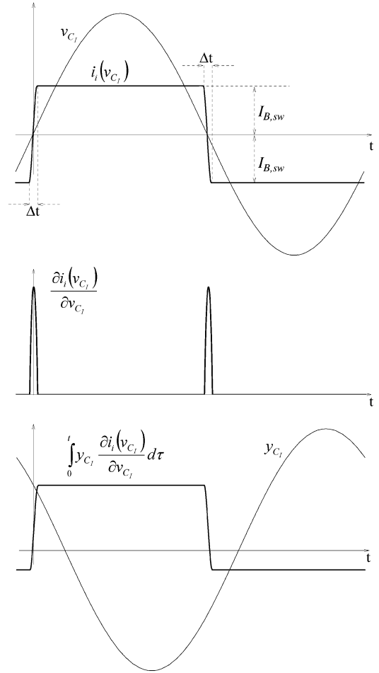
Fig. 7. Waveforms for the calculation of (88), where \partial i_i(v_{C_I})/\partial v_{C_I} is well approximated by two Dirac's delta functions.
