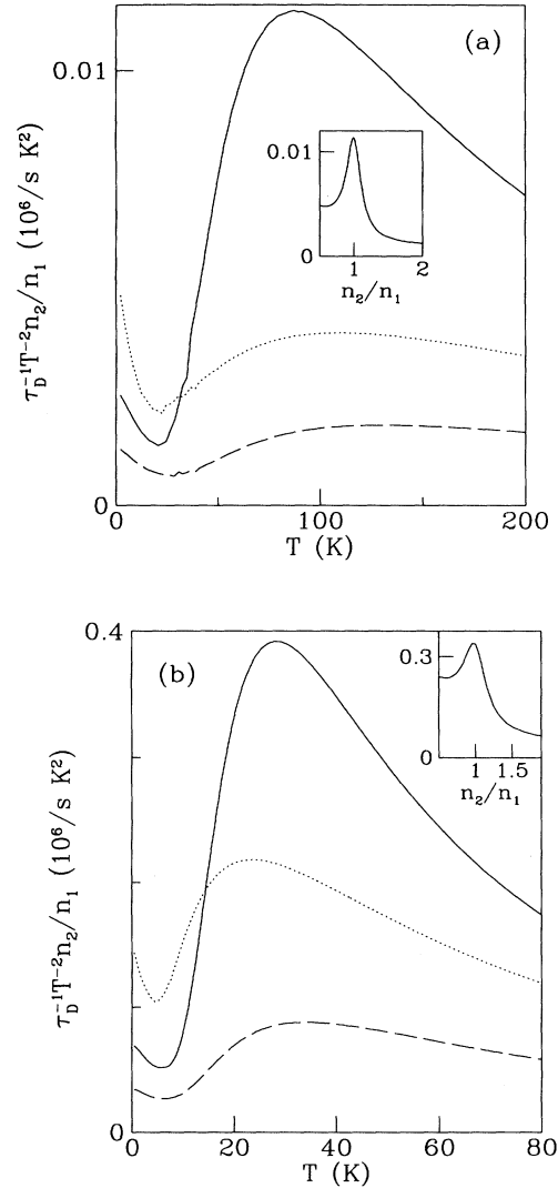
FIG. 5. The drag rate as a function of temperature, for well separation d = 800 \text{ \AA} and well width 200 \text{ \AA} , for densities (a) n_1 = 5 \times 10^{11} \text{ cm}^{-2} and (b) n_1 = 1 \times 10^{11} \text{ cm}^{-2} . The full, dashed, and dotted lines are for n_2/n_1 = 1, 2, and 0.5, respectively. Insets: drag rate as a function of relative density n_2/n_1 , when n_1 is fixed and n_2 is allowed to vary at (a) 80 K and (b) 20 K. The peaks at n_2/n_1 = 1 are evidence of plasmon enhanced drag.
