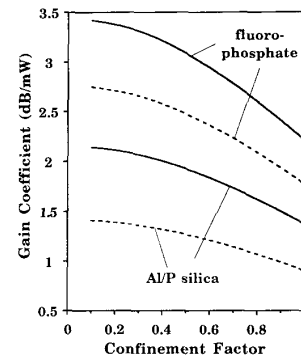
Fig. 9. Model predictions of gain coefficient as function of the erbium confinement factor for step-index fibers with an NA of 0.3. Curves are shown for codirectional (dashed curves) and bidirectional (solid curves) pumping of erbium-doped (a) Al/P-silica fibers pumped at 815 nm and (b) fluorophosphate fibers pumped at 802 nm.
