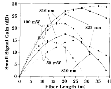
Fig. 3. Measured small-signal gain versus fiber length for different pump wavelengths. The erbium-doped Ge/Al/P-silica fiber has an NA of 0.18 and a cutoff wavelength of 940 nm. The signal wavelength is 1551 nm and the fiber is pumped codirectionally with 50 and 100 mW.
