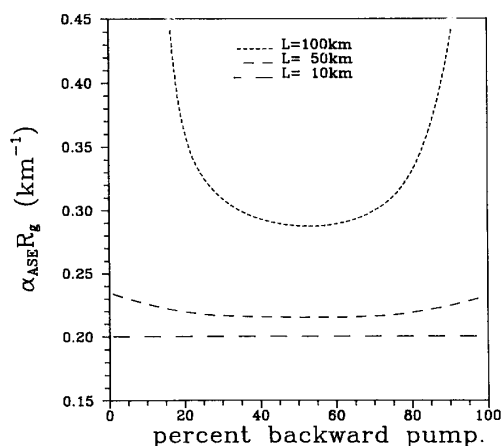
Fig. 3. The \alpha_{\text{ASE}} \cdot R_g product as a function of the backward propagating pump power relative to the forward propagating pump power, for three different fiber lengths.
