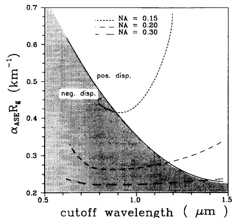
Fig. 2. The \alpha_{\text{ASE}} \cdot R_g product as a function of the \text{LP}_{11} cutoff wavelength for different values of the numerical aperture. The total fiber dispersion is negative in the gray area.
