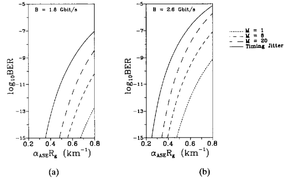
Fig. 5. The BER for (a) a 1.8-Gb/s and (b) a 2.6-Gb/s system, with the \alpha_{\text{ASE}} \cdot R_g product as parameter.
