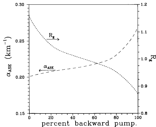
Fig. 4. \alpha_{\text{ASE}} and R_g as functions of the backward propagating pump power relative to the forward propagating pump power in a 50-km-long fiber with \text{NA} = 0.2 and cutoff wavelength equal to 1.22 \mu\text{m} .
