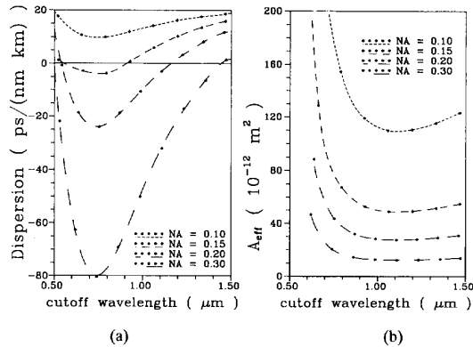
Fig. 1. (a) The total fiber dispersion and (b) the effective core area, both calculated for a step index profile as a function of the LP 11 cutoff wavelength with the numerical aperture of the fiber as parameter.
