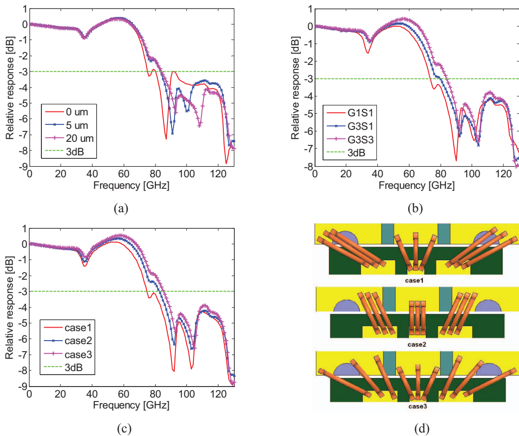
Figure 4. Simulated relative responses of chip-to-CBCPW wire-bonding transitions; (a) g = 0 \mu\text{m} , 5 \mu\text{m} and 20 \mu\text{m} ; (b) different numbers of bonding wires indicated by “ G_xS_y ”: x and y means the numbers of bonding wires connecting the ground and signal trace, respectively; (c) three typical arrangements of bonding wires as illustrated in (d). g = 20 \mu\text{m} in (b) and (c).
