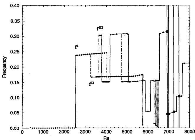
FIG. 9. Scenario of the rotating driven cavity problem. Stable solution ( \bullet ); branch (—); hysteresis (---); stable R-T frequency ( \bullet ); unstable R-T frequency ( \circ ); torus ( \cdots ); chaos (—).
