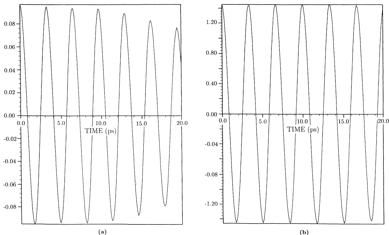
FIG. 13. One-phonon approximation to the intermediate coherent scattering function I'_{\text{coh}}(\kappa, t) , for the center of mass motion at two reciprocal lattice vectors of the herringbone lattice and temperature T = 10 K ( T/T_{\text{melt}} = 0.137 ), (a) at the wave vector \kappa = 1.703 \text{ \AA}^{-1} \hat{x} , which probes motion along \hat{x} at the Brillouin zone center and (b) at the wave vector \kappa = 2.95 \text{ \AA}^{-1} \hat{y} , which probes motion along \hat{y} at the Brillouin zone center.
