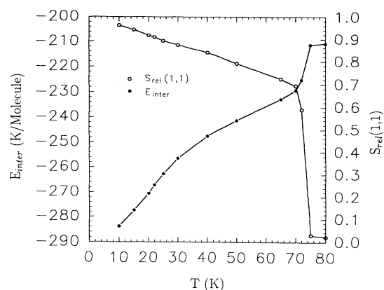
FIG. 5. Determination of the monolayer melting point. S_{rel}(1,1) is the relative structure factor with Miller indices (1,1) of the herringbone lattice with respect to the structure factor at 0 K, which was determined to be 126 862. S_{rel}(1,1) shows a strong drop in a temperature range of 70–75 K; from the inflection point, we assign the melting temperature as 73 K. This is consistent with the plot of the intermolecular potential energy per molecule, E_{inter} , also shown here. It has a sharp variation in the same temperature region with an inflection point at 73 K and a weaker inflection near the azimuthal disorder temperature, around 22 K. The latter transition is barely visible in the S_{rel}(1,1) structure factor.
