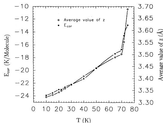
FIG. 7. The average corrugation energy per molecule E_{\text{cor}} and the average distance z of the molecules from the surface as a function of the temperature.
