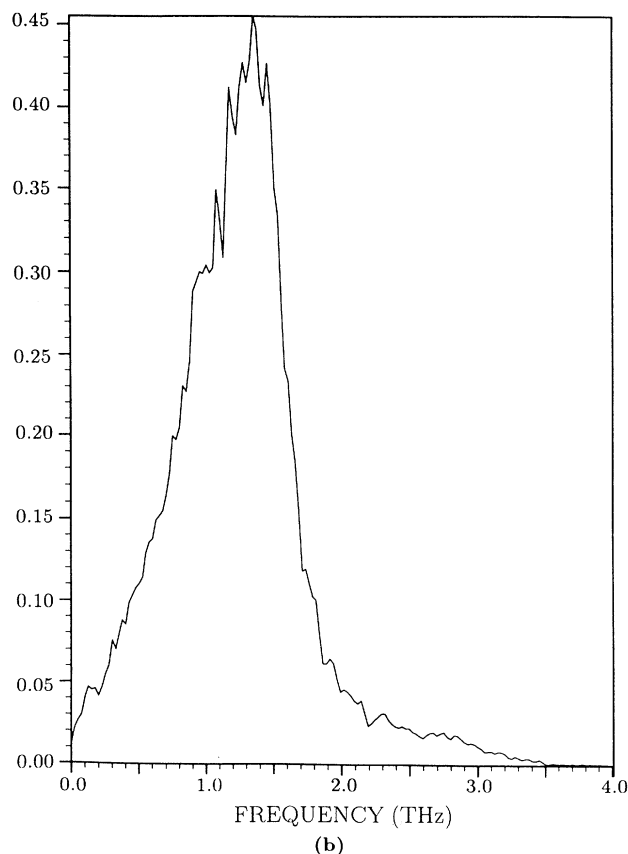
FIG. 11. Frequency spectra at T = 50 K ( T/T_{\text{melt}} = 0.685 ). (a) Translational motion of the molecules perpendicular to the surface, i.e., the bouncing mode. (b) The polar angle motion of the N-N bond, i.e., the tilting mode. (c) The lateral motion of the molecules in the x direction. (d) The lateral motion of the molecules in the y direction. (e) The azimuthal angle motion of the N-N bond.
