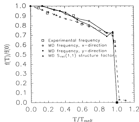
FIG. 15. Calculated gap frequencies f(T) for translational motion in the x and y directions relative to the frequency at 0 K, f(0) , and experimental inelastic neutron scattering results as a function of the relative temperature T/T_{\text{melt}} . Also shown as a dashed line is the relative structure factor S_{\text{rel}}(1,1) with respect to the structure factor S(1,1) at 0 K.
