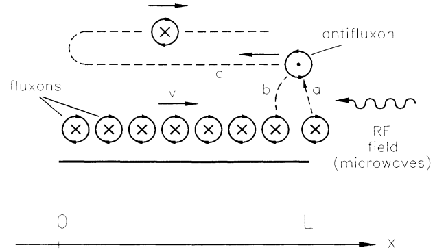
FIG. 4. A schematic representation of the dynamical processes in the junction induced by microwaves, corresponding to the satellite flux-flow steps appearing in I - V characteristics (for details see the text).
