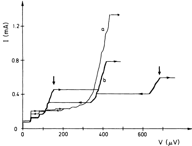
FIG. 2. Typical I - V curves for the junction B at I > 0 (curve a ) without and ( b ) with applied microwaves at f_{\text{ext}} = 68.0 GHz. Power level, P_a = 100 \mu\text{W} ; control current, I_m = -5.3 mA; temperature, T = 4.2 K. Satellite steps at voltages V_{-1} \approx 140 \mu\text{V} and V_{+1} \approx 680 \mu\text{V} are seen in curve b . The arrows indicate the satellite steps discussed in the text.
