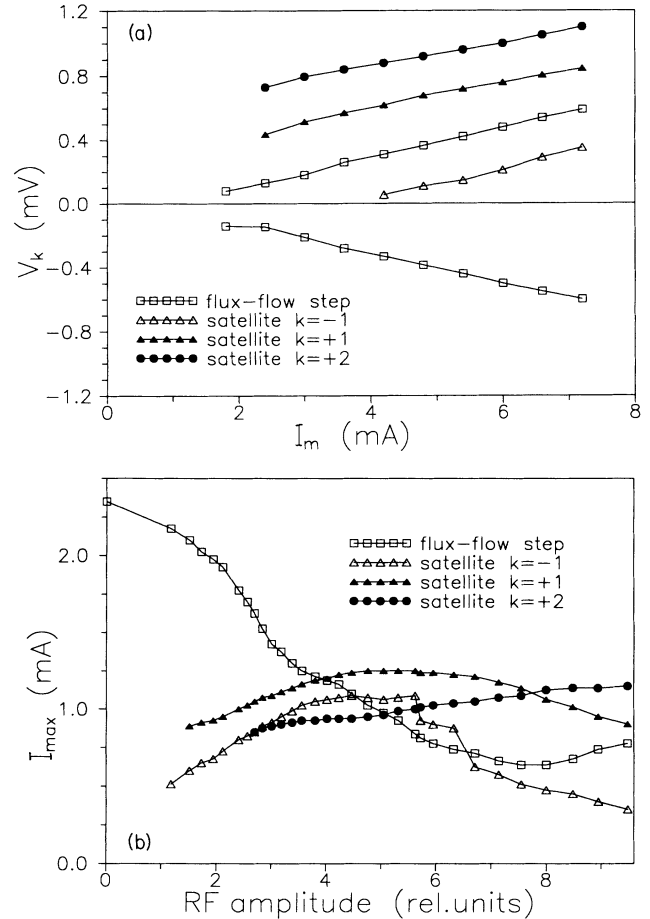
FIG. 3. (a) The dependence of the asymptotic voltage of the various steps on magnetic field (control current I_m ) at P_a = 3.0 \mu\text{W} and f_{\text{ext}} = 70.2 GHz for junction A . (b) Power dependence of the amplitude of the steps for junction A at I_m = -5.4 mA, f_{\text{ext}} = 75.4 GHz, and I > 0 ; T = 4.2 K.
