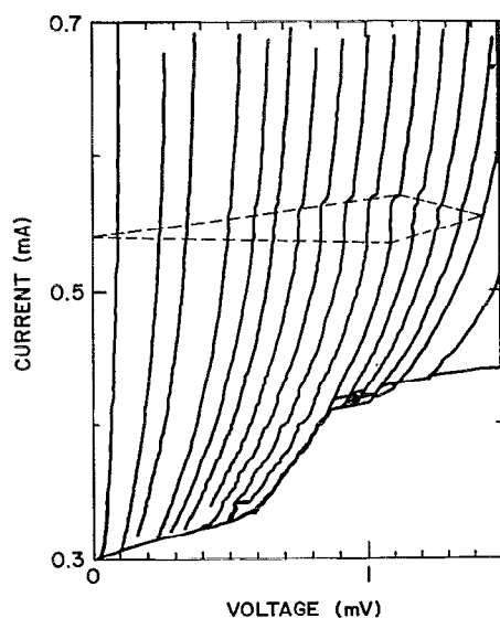
FIG. 3. I - V curves for a 16 junction sample (type B). The dashed lines indicate the locking range. Note that the current scale begins at 0.3 mA, and not at 0.
