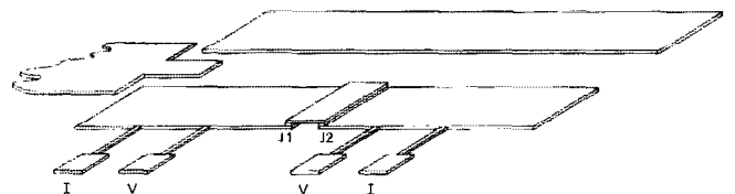
FIG. 1. Schematic drawing of the sample geometry. The junctions J1 and J2 are shown above the coplanar strip for clarity. In the actual samples, they were below.
