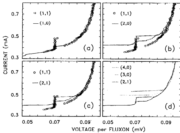
FIG. 2. Measured I - V curves for the different types of excitations in the two junction samples (type A). The voltages are shown normalized by the number of fluxons (voltage per fluxon) to facilitate comparison.
