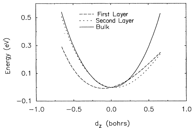
FIG. 2. The calculated potential felt by an atom in the first and second layer on a Cu(110) surface when it is moved perpendicular to the surface. The equivalent potential felt by a bulk atom is shown for comparison.
