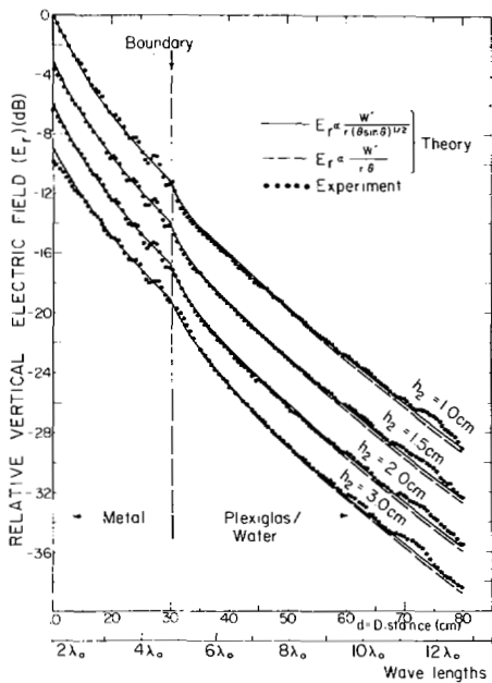
Fig. 5. Dipole excited groundwave field versus distance d (=a\theta) over two-section cylindrical (experimental) and spherical (theory) mixed paths composed of metal and Plexiglas over water. Frequency = 4.765 GHz ( \lambda_0 = 6.3 cm), boundary at d_1 = 30 cm, h_1 = 1.5 cm, and a = 125 cm ( 19.85 \lambda_0 ).
