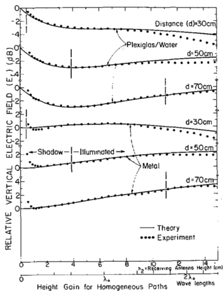
Fig. 3. Height gain data for propagation over cylindrical (experimental) and spherical (theory) homogeneous paths of either metal or Plexiglas over water. Frequency = 4.765 GHz ( \lambda_0 = 6.30 cm), h_1 = 1.5 cm, and a = 125 cm ( 19.85 \lambda_0 ).
