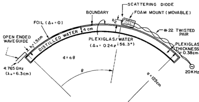
Fig. 1. Cross section of cylindrical Plexiglas water tank. Open-ended waveguide was used as transmitting antenna and modulated scattering diode (dipole) was used as probe to measure radial electric field.
