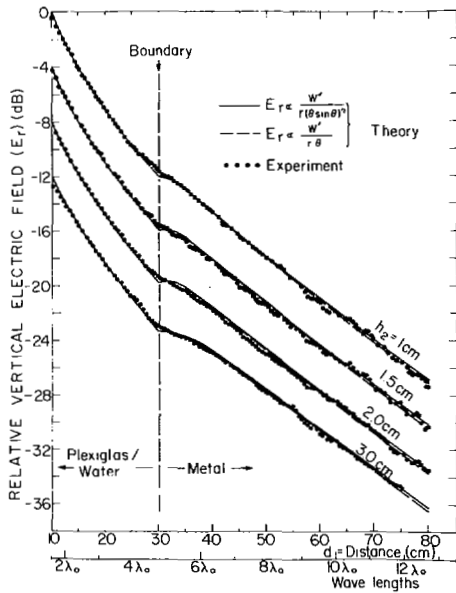
Fig. 4. Dipole excited groundwave field versus distance d (=a\theta) over two-section cylindrical (experimental) and spherical (theory) mixed paths composed of Plexiglas over water and metal. Frequency = 4.765 GHz ( \lambda_0 = 6.30 cm), boundary at d_1 = 30 cm, h_1 = 1.5 cm, and a = 125 cm ( 19.85 \lambda_0 ).
