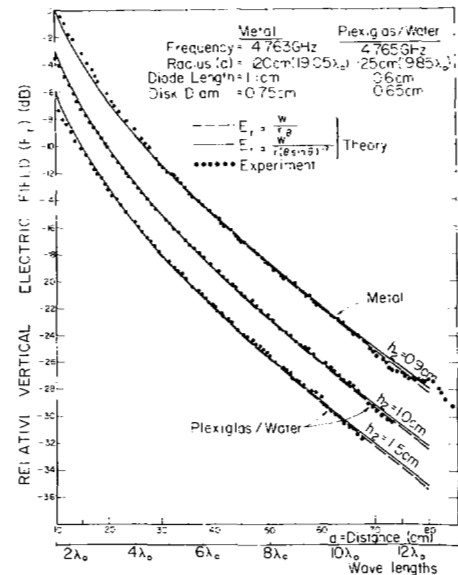
Fig. 2. Dipole excited groundwave field versus distance d ( = a\theta ) over homogeneous cylindrical (experimental) and spherical (theory) surfaces of metal ( \Delta = 0 ) and Plexiglas over water ( \Delta = 0.24 e^{i56.3^\circ} ), h_1 = 1.5 cm.
