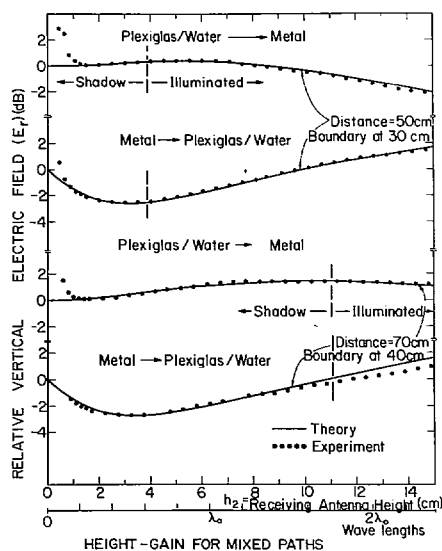
Fig. 6. Height gain for propagation over two-section cylindrical (experimental) and spherical (theory) mixed paths composed of metal and Plexiglas over water and vice versa. Frequency = 4.765 GHz ( \lambda_0 = 6.3 cm), boundary at 30 or 40 cm, h_1 = 1.5 cm, and a = 125 cm ( 19.85 \lambda_0 ).
