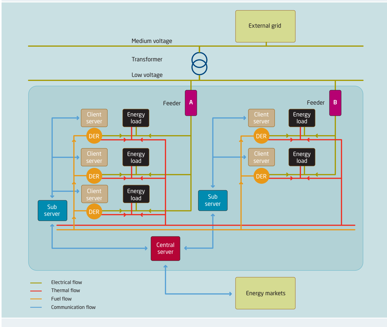
Figure 17 Topology of a generic VPP showing the integration of energy, electrical and information system.
