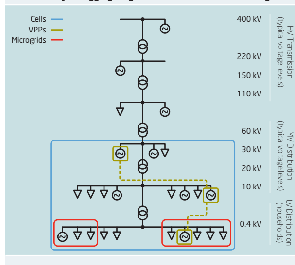
Different ways of aggregating units connected to distribution grid.
