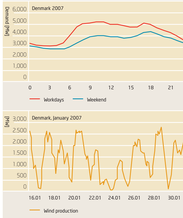
Figure 22 Average hourly consumption curves for Denmark 2007, and the variation of wind power production in the second half of January 2007.
