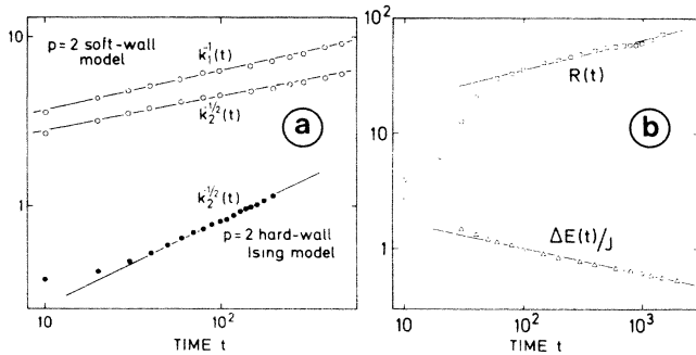
FIG. 2. (a) Log-log plot vs times of length scales derived from moments of the structure factor, Eq. (3). Results from quenches of the p=2 hard-wall Ising model (Ref. 18) are shown for comparison. The solid lines denote power laws, k_m^{-1/m} \sim t^n , with n=0.25 and n=0.50 for the soft-wall and hard-wall models, respectively. (b) Log-log plot vs time of the linear domain extension, R(t) , and the excess energy per rotor, \Delta E(t) . The solid lines denote the asymptotic power laws, R(t) \sim t^n and \Delta E(t) \sim t^{-n} , with the same exponent n \approx 0.2 . (Data for a 200 \times 200 lattice.)
