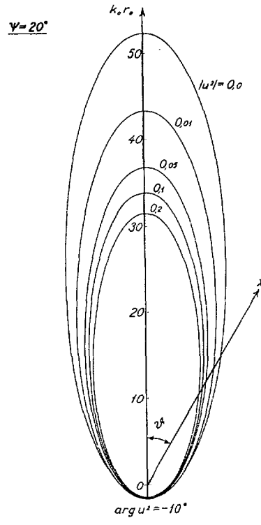
Fig. 7—First Fresnel zone for \psi = 20^\circ .
