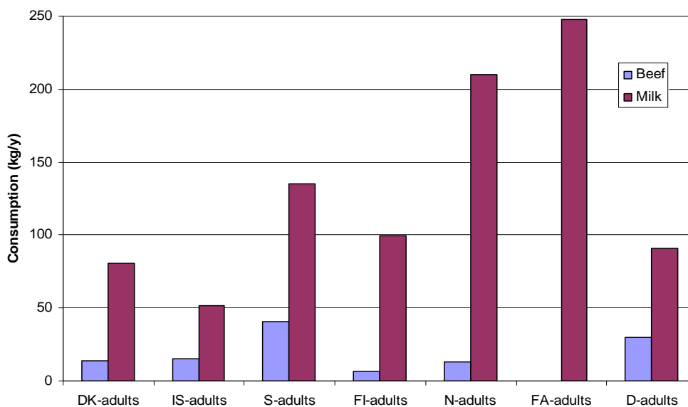
Figure 2. Consumption of beef and milk in the Nordic countries, and German ECOSYS defaults, D (averages for adults).
