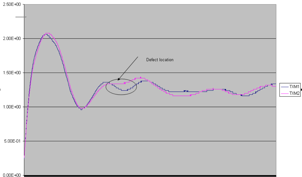
Figure 4. TDR trace for TXM1 and TXM2
