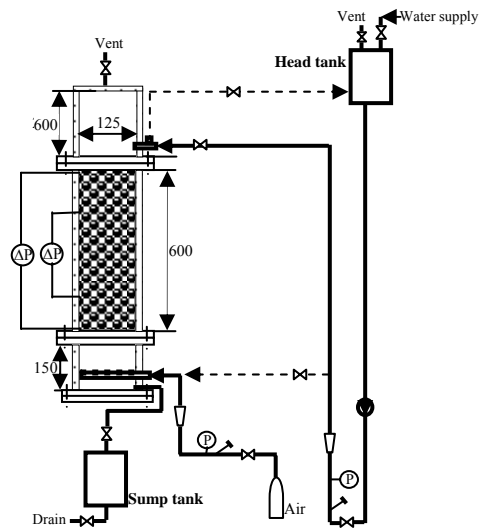
Figure 3. POMECA-FL Facility
