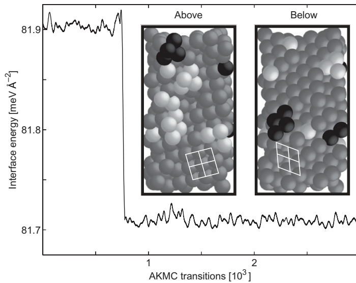
Figure 12. Energy as a function of AKMC transitions during the second significant annealing event. The energy curve has been smoothed by a weighted Gaussian average of the 20 transitions before and after the actual transition. The total process caused a lowering of structural energy by 0.08 eV, changing the interface energy from 81.9 to 81.7 meV Å -2 , and took place over 20 transitions. The insets show the \hat{X}\hat{Y} -planes of the GB as seen from above and below. Only GB atoms are shown, gray atoms were GB atoms both before and after the process, black atoms became GB atoms and white atoms obtained FCC coordination. The grids are imposed to help show that the interface below is a (111)-like surface, whereas above it is a (001)-like surface. In general, the reshaping is a flattening of the GB.
