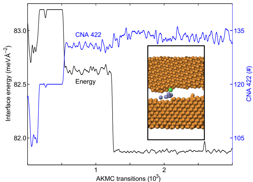
Figure 11. Energy and CNA422 as functions of AKMC transitions for the first significant annealing event. The curves were smoothed by a weighted Gaussian average of the 20 transitions before and after the actual transition. The event caused a structural energy lowering of 0.24 eV changing the interface energy from 83.2 to 82.6 meV Å -2 . A remarkable feature of the process is that an atom obtains a local HCP coordination. The transition where the HCP core is created involves five atoms being displaced by more than 0.5 Å. The core atom stays HCP coordinated throughout the rest of the simulation. The inset shows the creation mechanism where GB atoms are removed; exceptions are the five atoms that moved more than 0.5 Å, which are colored blue, and the GB atom that became HCP coordinated, which is green.
