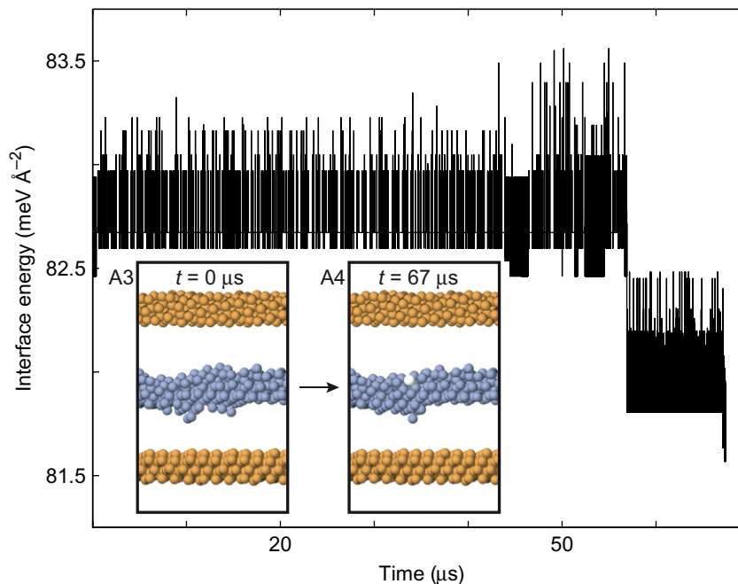
Figure 6. Interfacial energy as a function of time for the AKMC simulation. Two events lower the energy significantly. The first occurs after 55 \mu\text{s} and is due to the creation of a locally HCP-coordinated atom. The energy decrease at 66 \mu\text{s} is a series of approximately 20 transitions resulting in a flattening of the GB. Inset (A3) shows the initial configuration for the AKMC simulation, which corresponds to figure 3(A2) that has been relaxed. Inset (A4) is the final low-energy configuration. In the insets, all FCC-coordinated atoms are removed. The white atom in the boundary is the one with local HCP coordination.
