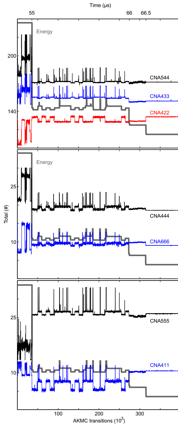
Figure 9. CNA curves for abundant pairs, excluding the CNA421 FCC-like pairs. The curves have been smoothed by a weighted Gaussian average of the 50 transitions before and after the actual transition. The bold gray curve is a schematic representation of the energy. Most of the curves fluctuate in phase with the energy. However, an exception is the CNA422 HCP-like structure—an indication that this local structure is favored. The CNA555 and energy curves are out of phase at the two significant energy lowering events, indicating an increase in local icosahedral order.
