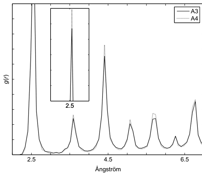
Figure 8. RDFs for the MD-annealed configuration relaxed to 0 K, figure 6(A3), and the final low-energy configuration for the AKMC annealing, figure 6(A4). The result of the AKMC annealing is that the spikes and valleys become more distinct, indicating a transformation toward an ordered FCC structure.
