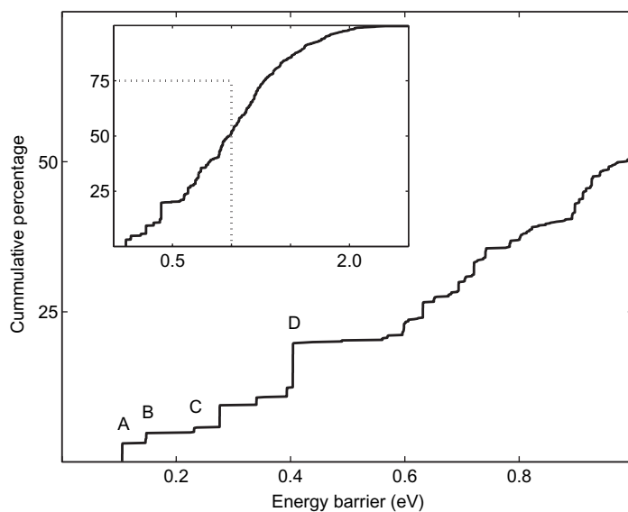
Figure 1. Distribution of 1000 SP searches. The inset accounts for all SPs determined; the dashed rectangle marks the region shown in the major plot. The mechanism labeled A involves two atoms ( \geq 0.5 Å) and accounts for 3.1%. B involves 4 atoms and accounts for 1.7%, C involves four atoms and accounts for 0.9%. The mechanism labeled D is marked due to its abundance; it involves four atoms and accounts for 7.3%. As the lowest energy mechanism is determined once for every 33 searches, the criterion of 200 converged SPs should be more than sufficient to ensure a determination of the most significant mechanism.
