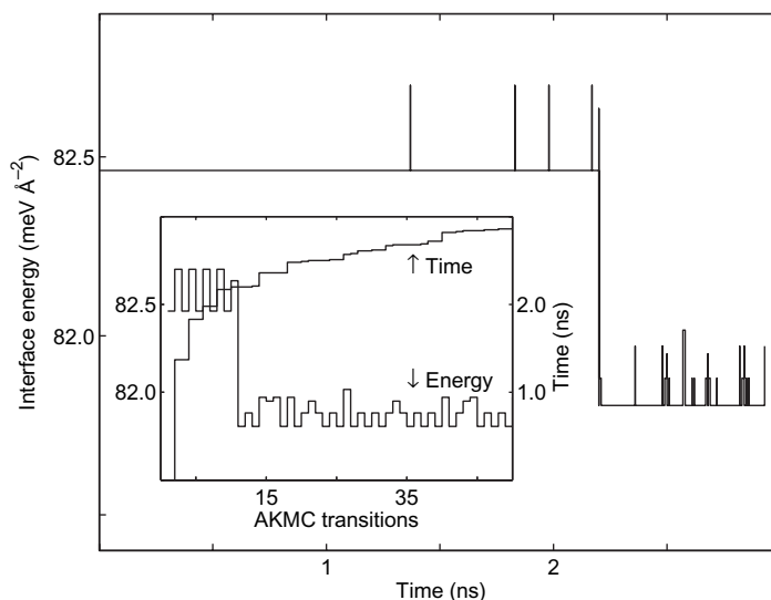
Figure 5. Plot of energy versus time for AKMC dynamics. The inset depicts energy and time as functions of AKMC transition number. Time does not evolve linearly but in bursts; an example is the first transition at 1.4 ns. A slow transition creates a plateau on the energy versus time graph whereas spikes are formed when transitions are rapid.
