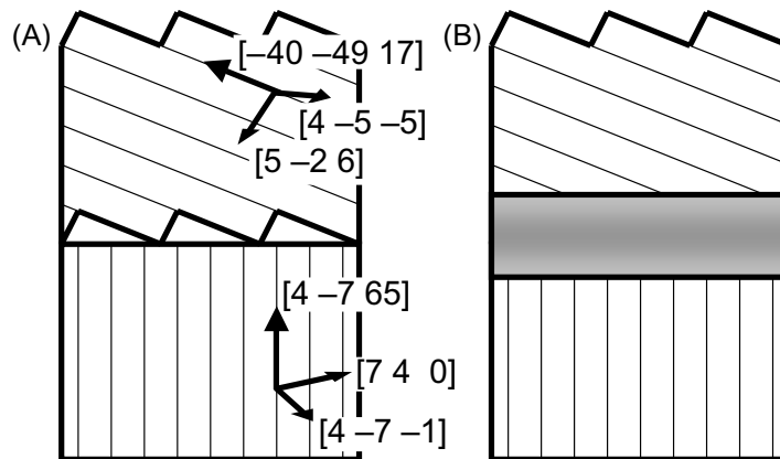
Figure 2. Schematics of the initial structures. (A) The thin GB is a sharp interface between two single-crystalline domains. (B) The wide GB is an amorphous slab of six atomic layers separating the domains.
