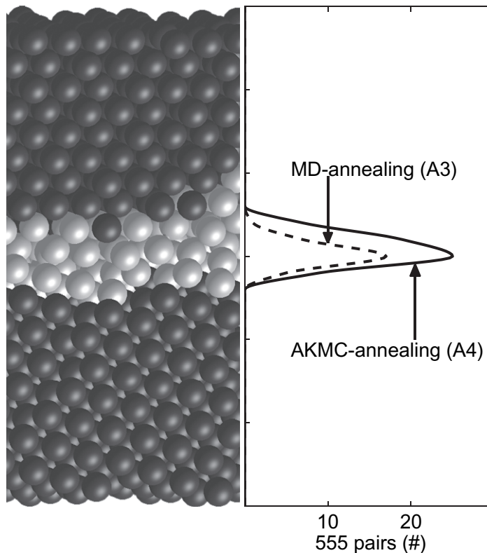
Figure 10. Layered CNA for CNA555 pairs tracing out the evolution of local icosahedral structure. A number of such pairs are partitioned into 31 layers along the \hat{Z} -axis to form a histogram. The area under these curves is 30 for the MD-annealed structure and 60 for the AKMC-annealed structure. It is remarkable that the curves rise most rapidly when the boundary is approached from below. The plot shows that changes toward CNA555 coordination occur primarily in the upper part of the interface.
