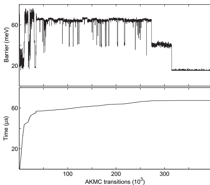
Figure 13. Barrier height and accumulated time as functions of AKMC transitions. The barrier curve is a Gaussian average of the 50 iterations before and after the actual transition. It is counterintuitive in that the barrier height decreases over the course of the simulation.
