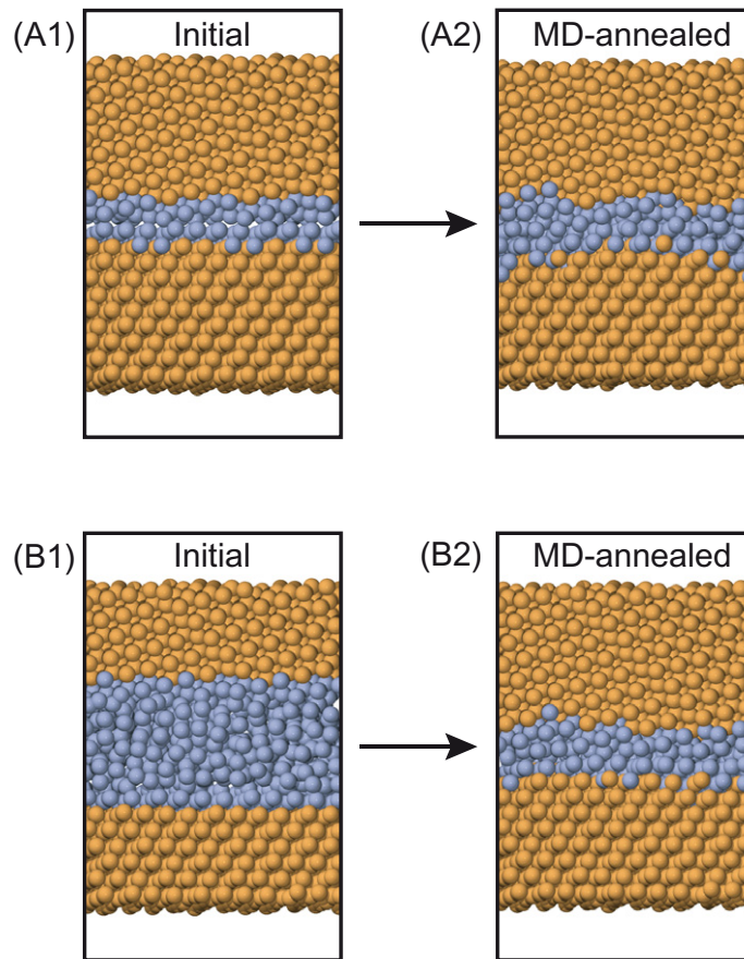
Figure 3. The effect of annealing first at 300 K and then at 135 K using MD. The structures and interfacial energies are (A1) initial thin GB, 141.1 \text{ meV } \text{\AA}^{-2} , (B1) wide GB, 2481.2 \text{ meV } \text{\AA}^{-2} , (A2) annealed thin GB, 82.4 \text{ meV } \text{\AA}^{-2} and (B2) wide GB, 83.9 \text{ meV } \text{\AA}^{-2} . Copper-colored atoms are FCC coordinated and blue atoms are GB atoms.
