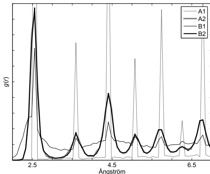
Figure 4. RDFs for the initial and annealed configurations. The analysis accounts for the subset of atoms that are initially GB atoms in the wide boundary—the blue atoms in figure 3(B1). Curves (A1) and (B1) are the initial thin and wide GBs at 0 K. Curves (A2) and (B2) are after MD annealing. The annealed configurations (A2) and (B2) have similar distributions between the two initial configurations, which indicates that a similar annealed GB structure has been obtained from both our thin and wide initial structures.
