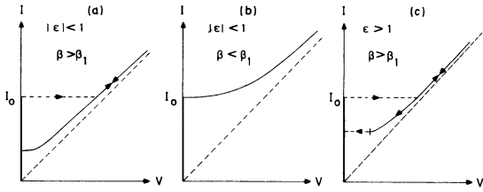
FIG. 3. Typical IV curves.
