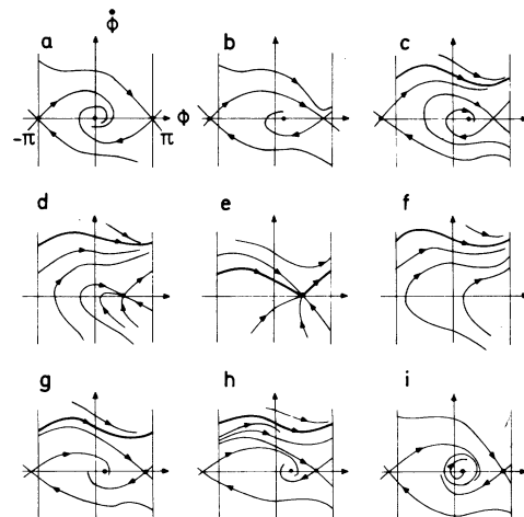
FIG. 2. Qualitative phase-plane portraits. The letters correspond to the regions in Fig. 1 and are discussed in the text.
