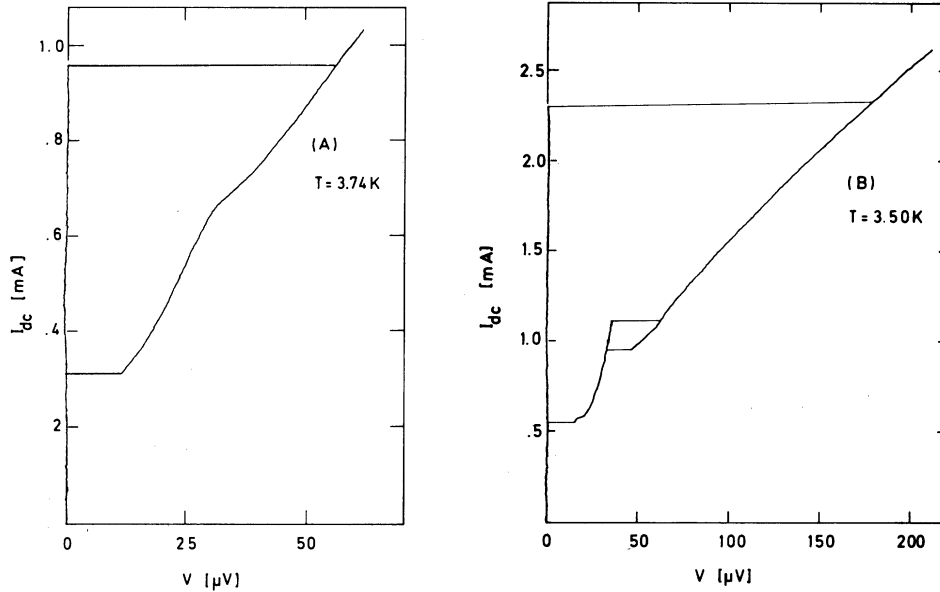
FIG. 4. Experimental IV curves obtained on a single Sn-O-Sn tunnel junction at two different temperatures.
