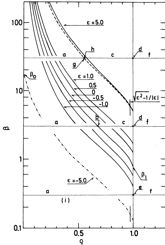
FIG. 1. Parameter space decomposition. The bifurcation curves \rho = \rho_c(\beta, \epsilon) are shown by heavy lines for values of \epsilon as indicated. The dashed line shows the curve \rho = \rho_d(\beta, \epsilon) for \epsilon = 5 and the dash-dotted line shows qualitatively the bifurcation for \epsilon = -5 . The letters correspond to the different pictures in Fig. 2.
