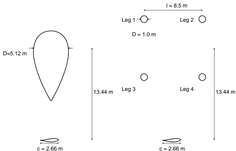
Figure 5. Upwind and downwind configurations for the 40%, 60% and 80% radius blade sections.
