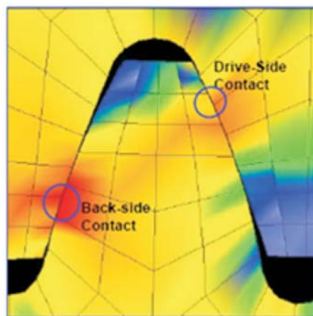
Figure 126. Example of a double contact situation where the backside of the teeth are also in contact.
