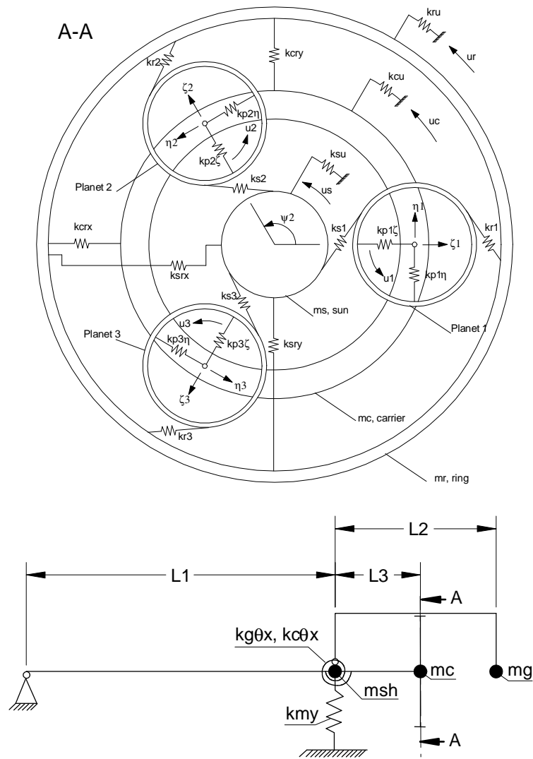
Figure 125. Dynamical model used to investigate the drive train dynamics with particular focus on gear teeth and bearing forces.
