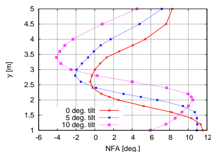
Figure 42. Effect of tilt on the nacelle flow angle (NFA) as a function of vertical distance.
