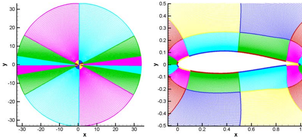
Figure 88. Mesh configuration.
