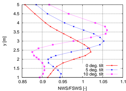
Figure 41. Effect of tilt on the nacelle wind speed (NWS/FSWS) as a function of vertical distance.
