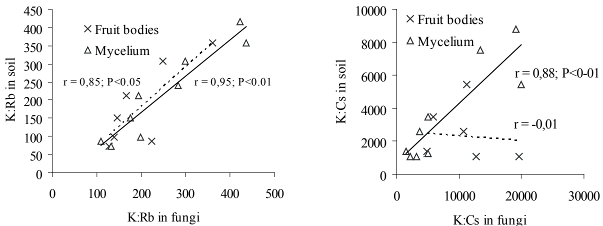
Figure 1. Relationships between K, Rb and Cs concentration, mg per kg d.w. in fungal mycelium and fruit bodies of fungi.
