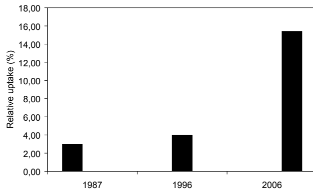
Figure 3. The relative amount of 137 Cs in Scots pine ( Pinus Sylvestris L. ) of the total load.
