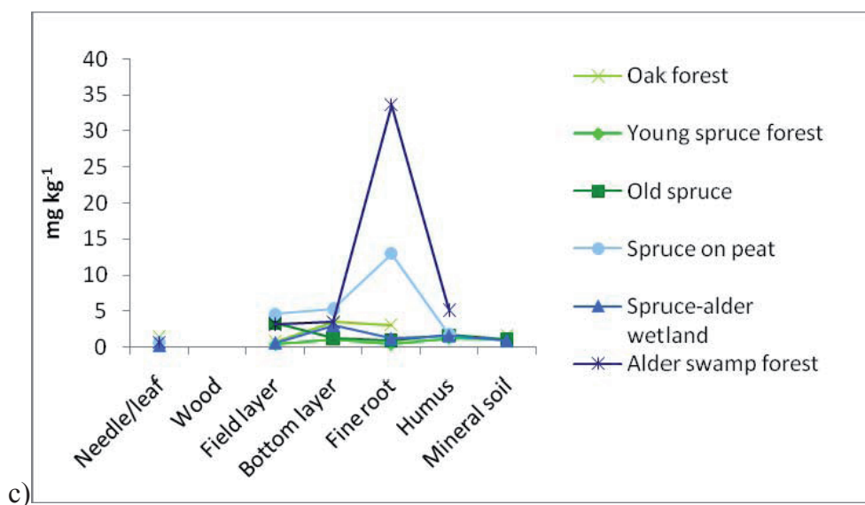
Figure 3. Measured concentrations of a) thorium, b) uranium and c) iodine in the different compartments of six forest ecosystems.
