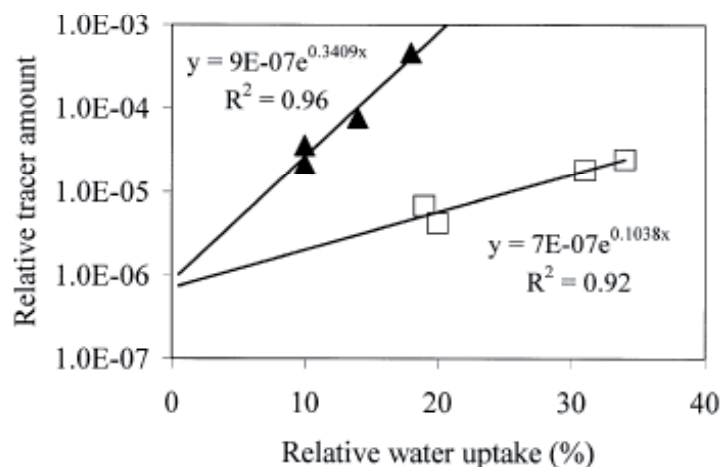
Figure 4. The relative water uptake from 0–10 cm ( 134 Cs) and 10–25 cm ( 22 Na) as a function of the amount of 22 Na and 134 Cs in xylem sap relative to the amount injected, for the treatments irrigation and desiccation in July 1995 at Åheden.
