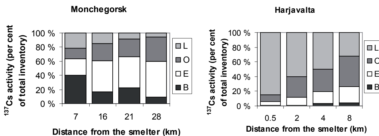
Figure 1. Distribution of ^{137}\text{Cs} among litter (L), organic (O) and mineral layers (E and B) along the pollution gradient in Monchegorsk (Bunzl et al. 2001) and Harjavalta (Outola et al. 2003).
