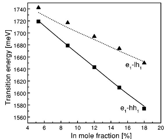
FIG. 7. Measured e_1-hh_1 (squares) and e_1-lh_1 (triangles) transition energies of S3, compared to calculated values for the heavy (solid line) and light hole (dotted line) using Eq. (6) for the band gap energy.
