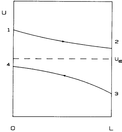
FIG. 2. A schematic picture of the periodic fluxon velocity vs position x in the overlap Josephson junction ( 0 < x < L ). From 1 to 2, the fluxon decelerates toward the power balance velocity u_\infty . At x = L , the fluxon is reflected as an antifluxon with less energy. From 3 to 4, the antifluxon accelerates towards the velocity u_\infty . At x = 0 , the antifluxon is reflected as a fluxon with larger energy.
