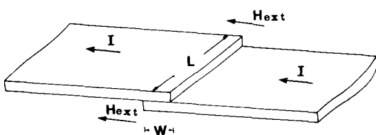
FIG. 1. The geometry of the overlap Josephson junction. Note that bias current is perpendicular to the length of the junction, and that the external magnetic field is applied in the direction of the current.
