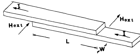
FIG. 5. The geometry of the inline Josephson junction. Note that the bias current is parallel to the length of the junction, and that the external magnetic field is applied perpendicular to the current.
