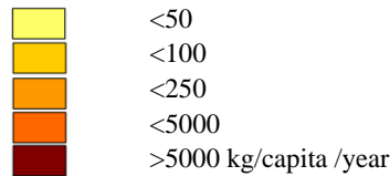
Figure 3.10: Hazardous waste
