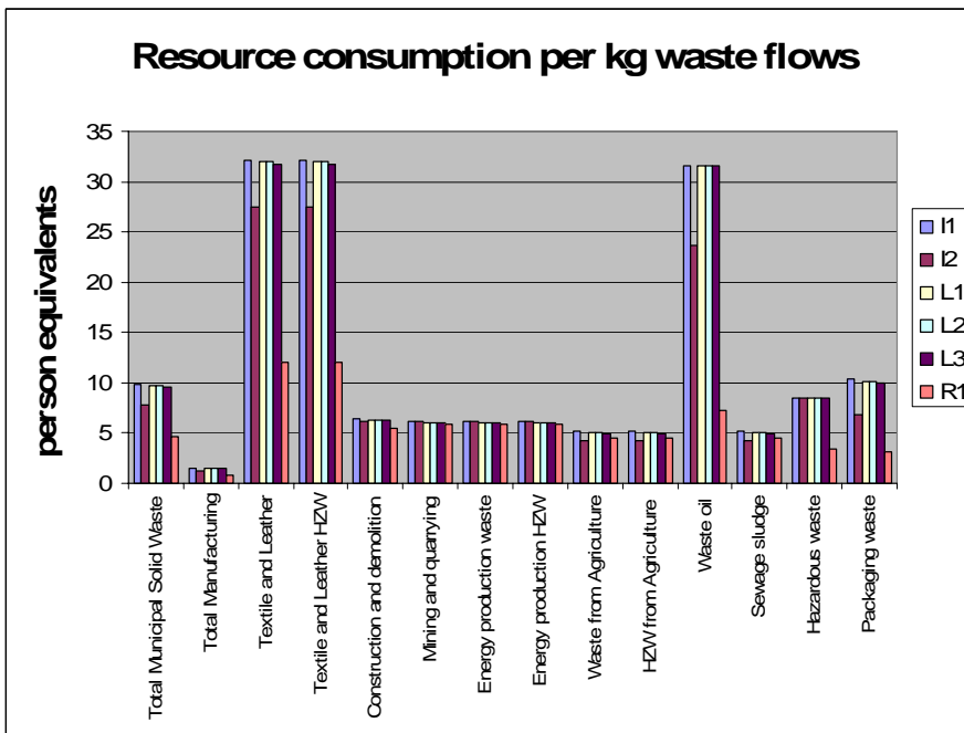
Figure 4.16: The normalised consumption of resources from 1 kg of waste flows with a material distribution as presented in table 4.13.
