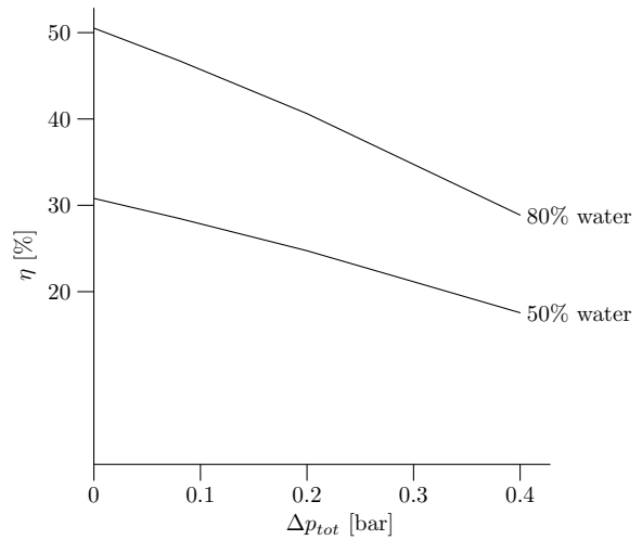
Figure 7: The Influence of Pressure Loss on Cycle Efficiency (LHV basis) for 50% and 80% Water Content in Fuel. (The pressure Loss, \Delta p_{tot} , is the total Pressure Loss in the cycle. The pressure losses in each of the Flows through Heat Exchanger Cold Side, Combustion, Heat Exchanger Hot Side and Dryer are equal.)
