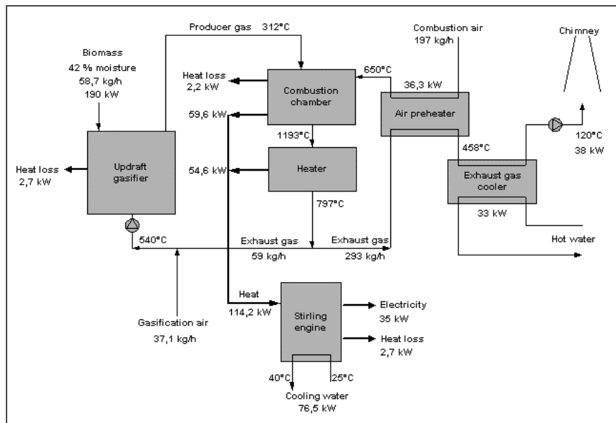
Figure 5: Results from the simulation of the demonstration plant. The thin lines represent mass flows in the system and the thick lines illustrate energy flows.
