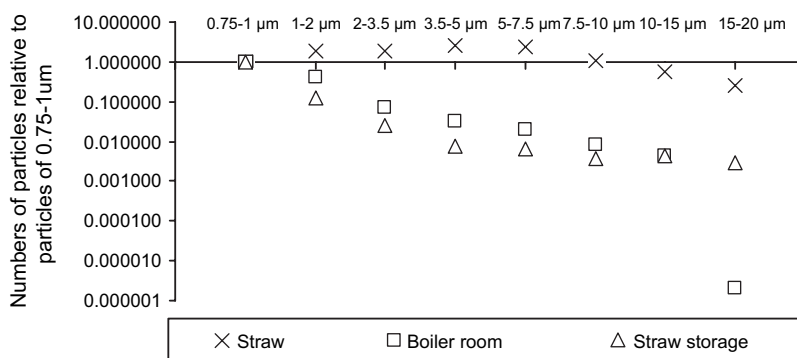
Fig. 1. Number of particles of different size categories relatively to numbers of particles with aerodynamic diameters between 0.75 and 1 µm present in the boiler room and in the straw storage for 9 days in March 2006 and released from a straw sample. Particles in the boiler room and particles released by the straw have been measured using a GRIMM particle counter and particles in the straw storage have been measured using an APS.
