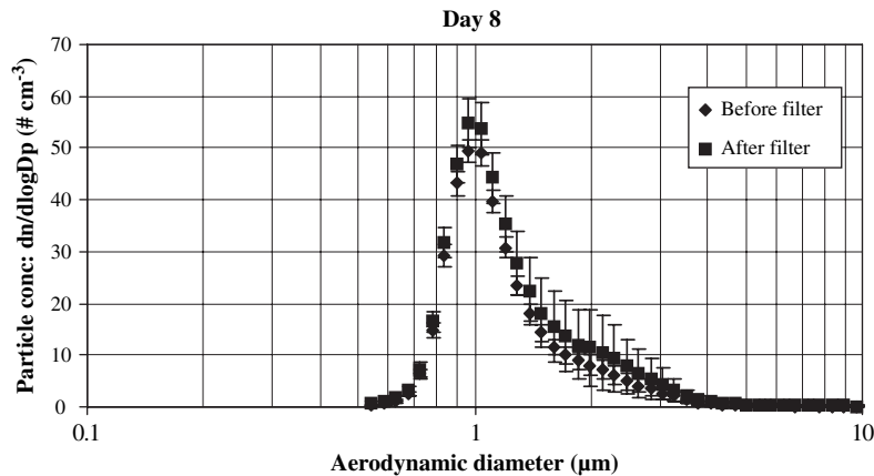
Fig. 5. Performance of the prefilter on day 8, determined by the APS. Error bars represent standard deviations.
