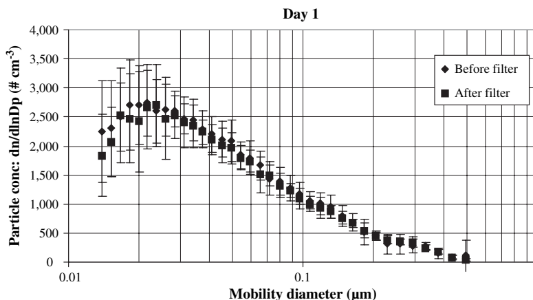
Fig. 2. Performance of the prefilter on Day 1, determined by the SMPS. Error bars represent standard deviations.
