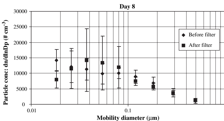
Fig. 3. Performance of the prefilter on Day 8, determined by the SMPS. The number concentration of four adjacent channels is pooled. Error bars represent standard deviations.
