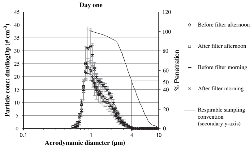
Fig. 4. Performance of the prefilter on Day 1 in the morning and afternoon, determined by the APS. Error bars represent standard deviations. The respirable sampling convention is also plotted (secondary y-axis).
