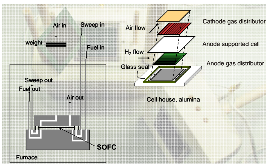
Fig. 4 Setup for testing SOFCs; Left: Alumina cell house (grey body) with gas supply and sealings; Right: Sandwiching of cell between auxiliary layers (gas distribution and current collection layers) and sealing bars
