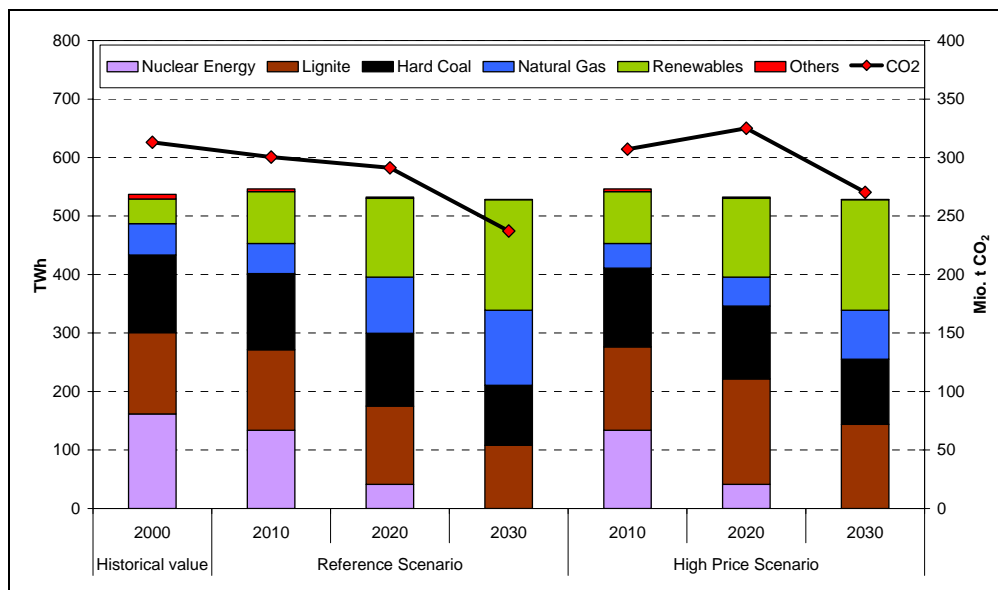
Figure 4: Net electricity generation and CO 2 emissions for the reference and high price scenario assuming current ETS allocation provisions
