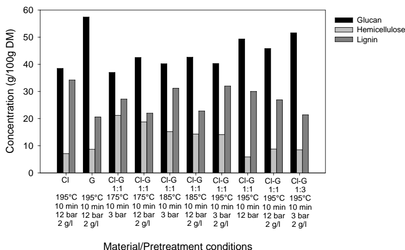
Figure 3 Glucan, hemicellulose, and lignin content in the fiber fraction of wet oxidised clover (CI), grass (G), and clover-grass mixtures (CI-G).
