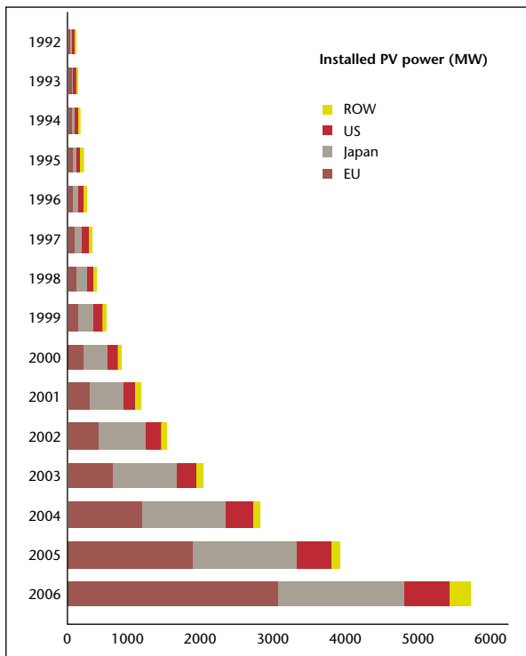
Figur 28: Cumulative installed PV capacity.
