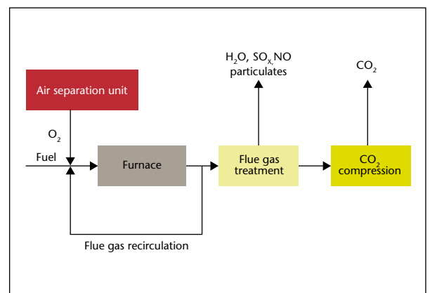
Figure 33: General flow sheet for oxy-fuel combustion [3].
