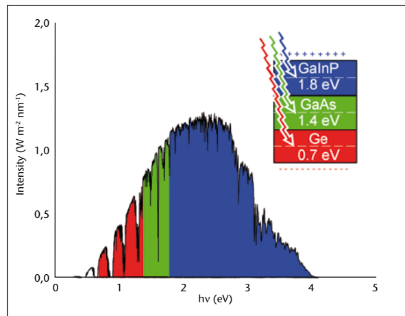
Figure 26: This triple-junction PV cell has three semiconductor layers, each of which absorbs a different part of the solar spectrum. Photons with energies higher than the band gap of 1.8 eV are absorbed by the GaInP layer. Photons with energies below 1.8 eV pass through the GaInP to the GaAs layer below, which absorbs visible light from 1.4 to 1.8 eV. Near-infrared light passes through the GaAs and is in turn absorbed by the bottom Ge layer. The layers are connected in series.
