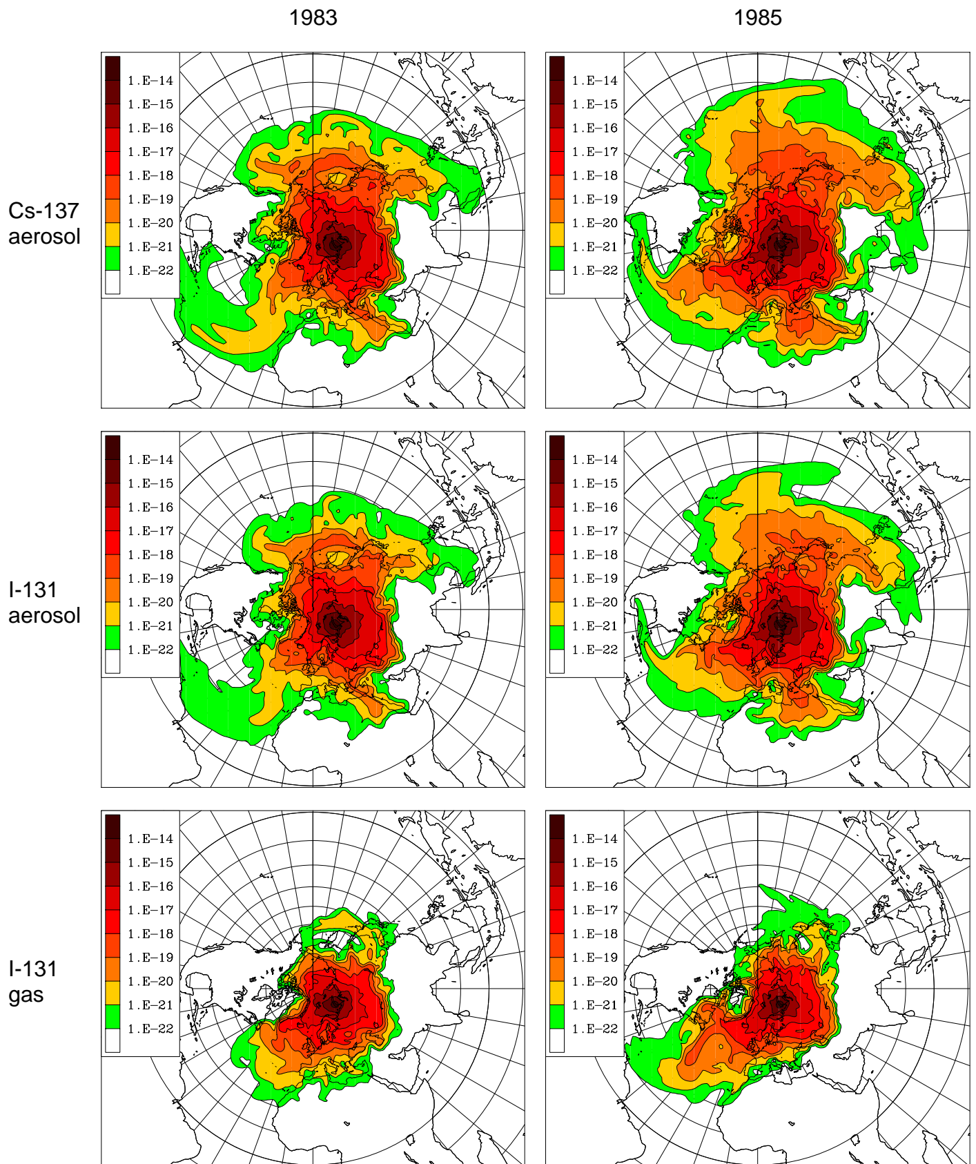
Figure M7. Novaya Zemlya, time-integrated air concentration
