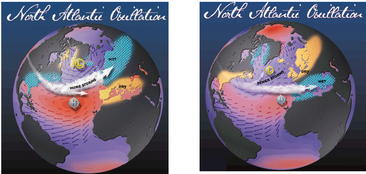
Figure 1. Weather patterns corresponding to a positive (left) and a negative (right) NAO index. Figure reproduced with permission from Hurrell et al. (2003).
