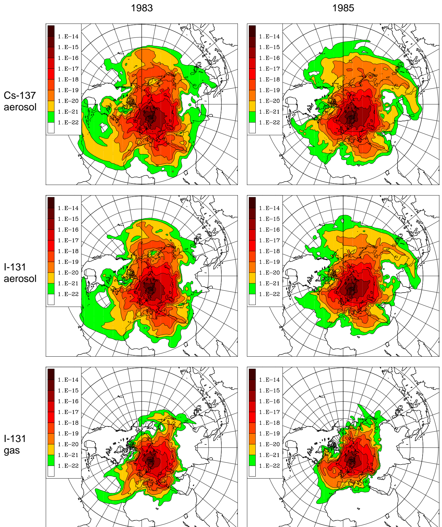
Figure M3. Kola, time-integrated air concentration
