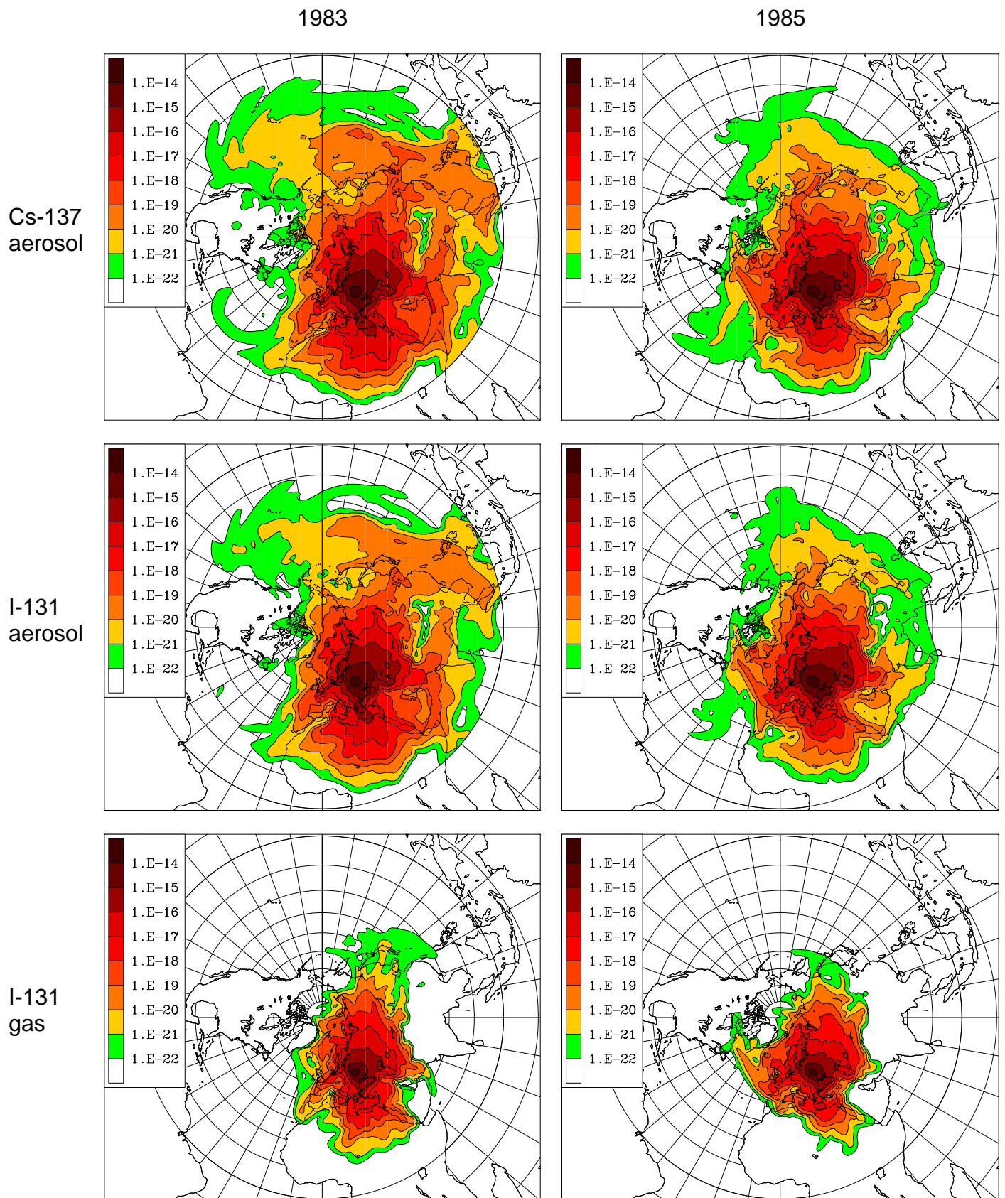
Figure M1. Chernobyl, time-integrated air concentration
