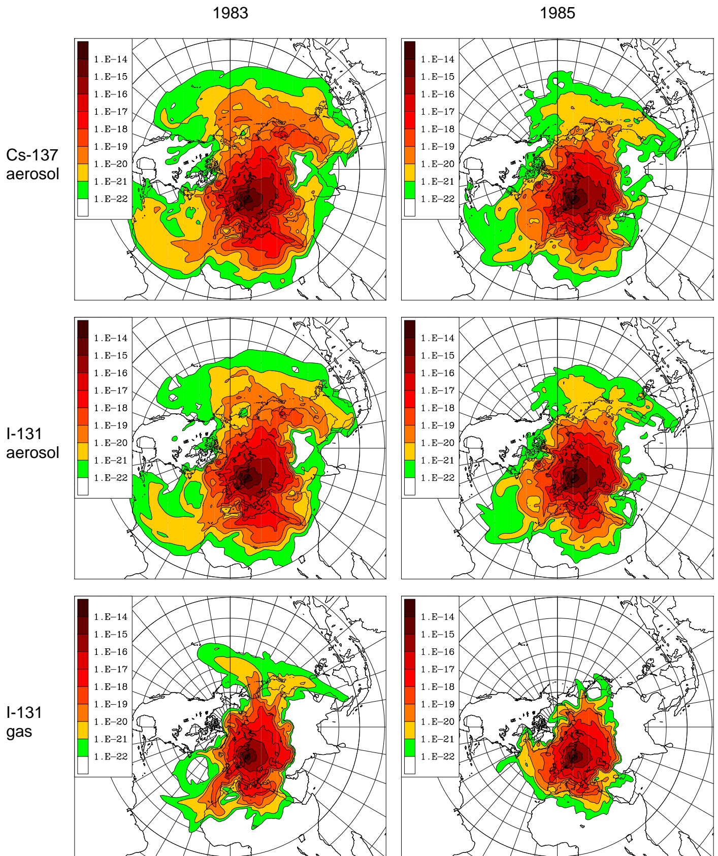
Figure M5. Leningrad, time-integrated air concentration
