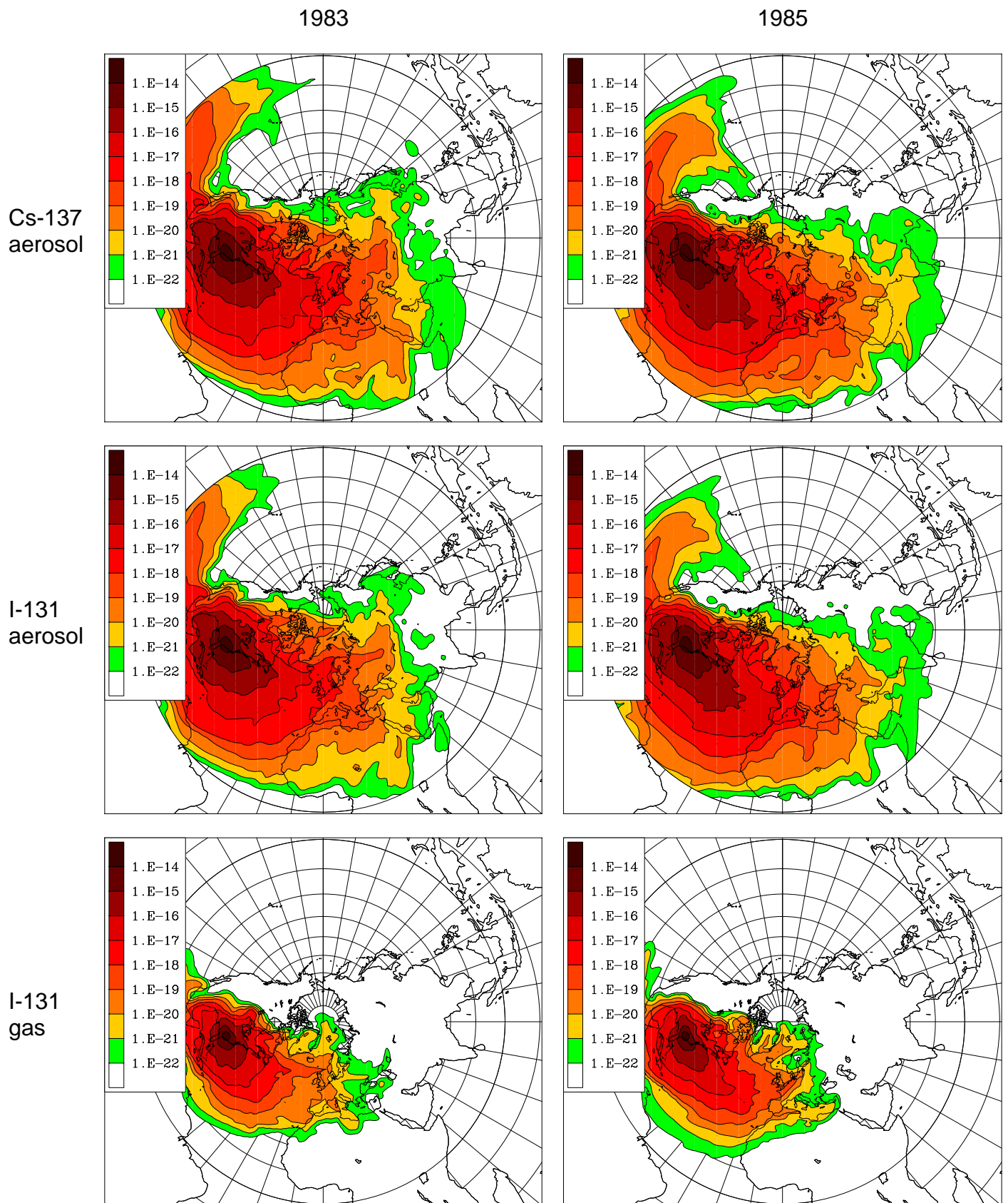
Figure M13. Savannah River, time-integrated air concentration
