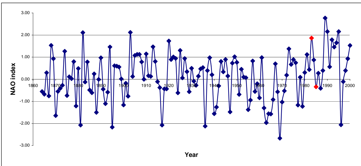
Figure 2. NAO index for the period 1864–2000 AD. The selected years 1983 and 1985 are marked in red colour.
