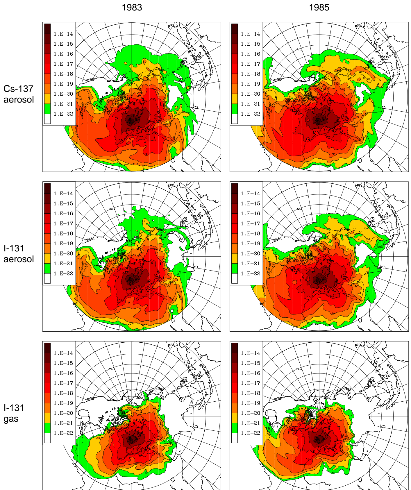
Figure M9. Sellafield, time-integrated air concentration
