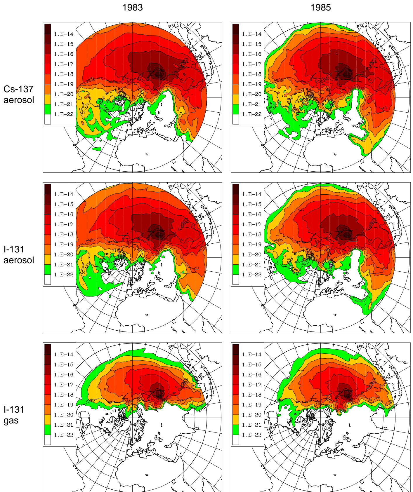
Figure M11. Sinpo, time-integrated air concentration
