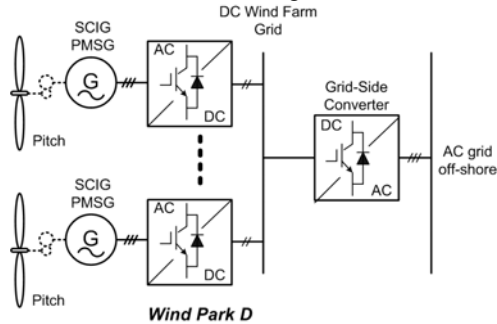
Figure 25. Wind farm with common DC grid based on variable speed wind turbines with full scale power converter.
