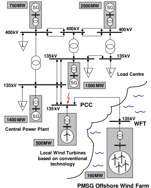
Figure 9: Generic power transmission system model
