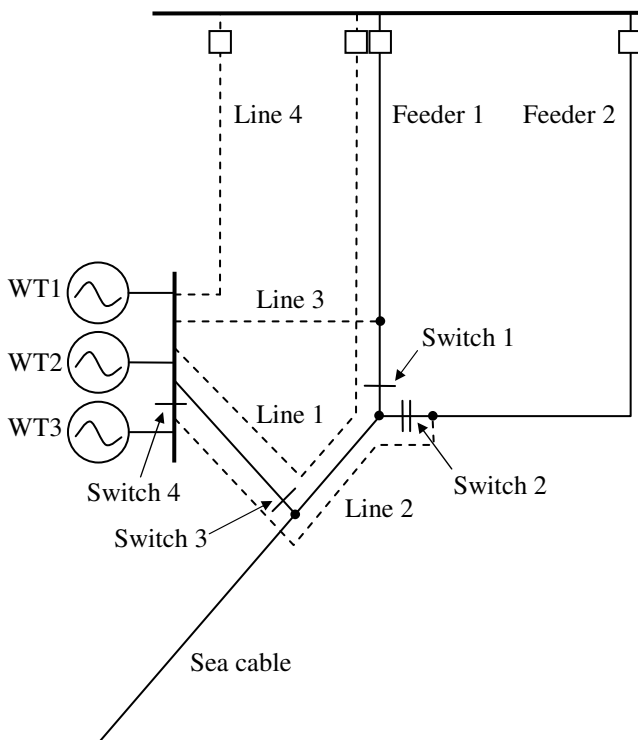
Figure 2. Example network.
