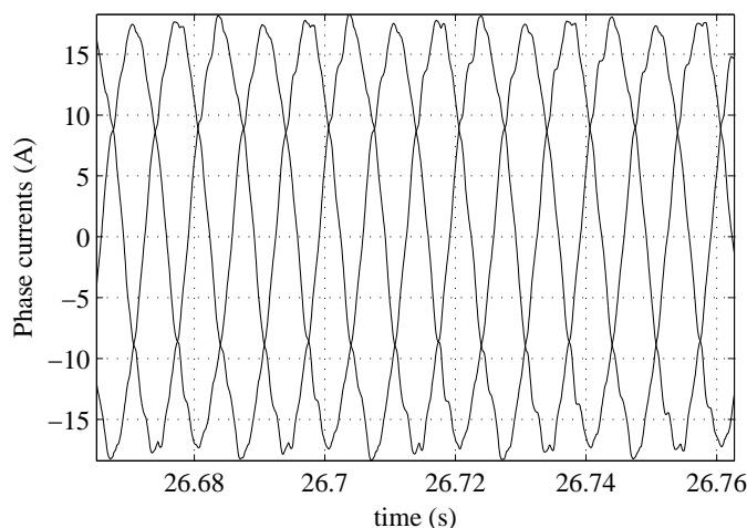
Fig. 10. Steady-state phase currents - no-load current
