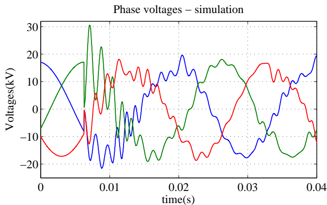
Fig. 14. Phase voltages during transient - simulation
