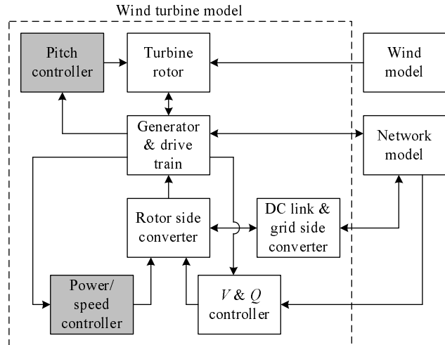
Fig. 1. General structure of model of wind turbine with DFIG
