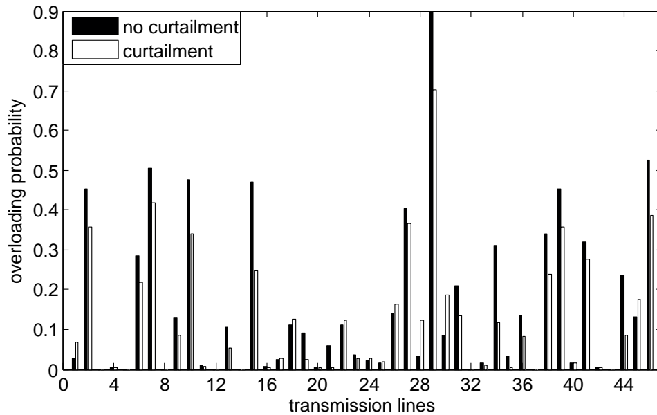
Fig. 7: Overloading probabilities of the transmission lines
