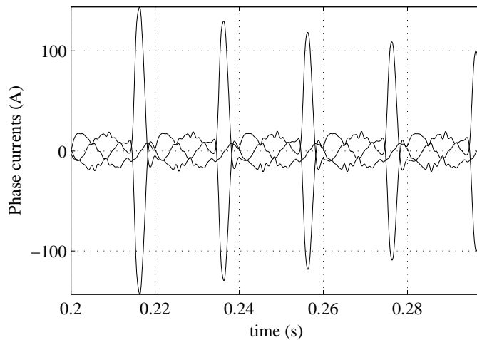
Fig. 9. Phase currents during the transformer energizing transient
