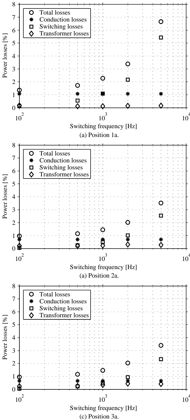
Figure 7. Loss distribution for IGBT module 1 using duty cycle control at the average wind speed 7.2 m/s.
