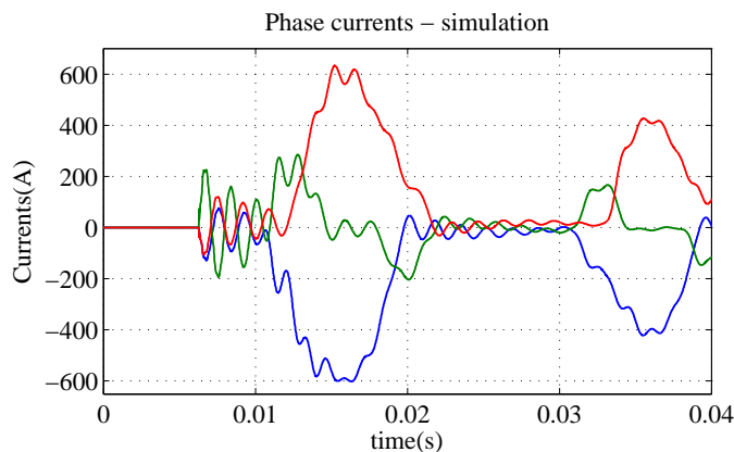
Fig. 15. Phase currents during transient - simulation
