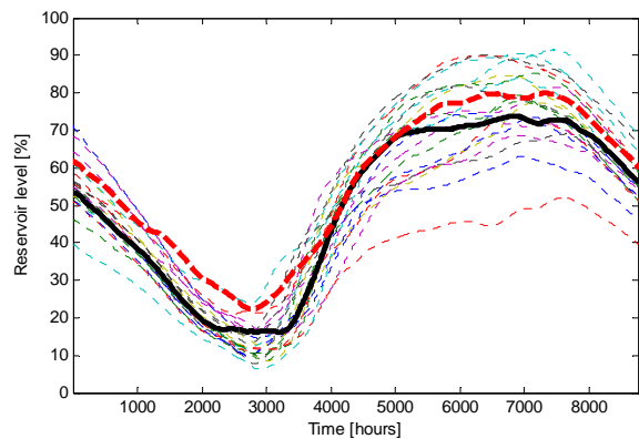
Figure 6. Simulated hydro reservoir level in Case A (15 TWh load increase), using 21 consecutive years of inflow data. The solid thick line is the median level. The dotted thick line is the median level for the reference case.
