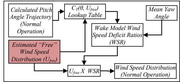
Figure 2-7: Normal Application of the Wake Model
