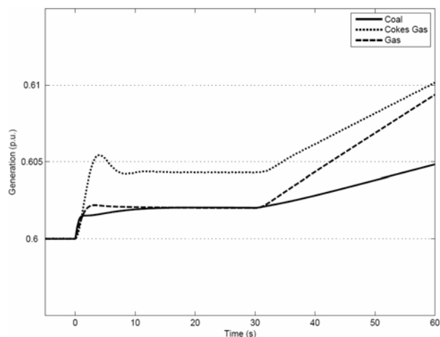
Fig. 3. Simulated responses of three generation unit responses to frequency and a operating set-point steps
