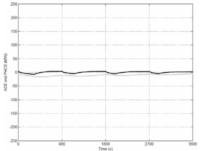
Fig. 4. Area Control Error (ACE, black line) and Processed Area Control Error (PACE, grey line) of the Dutch control zone with 0 GW wind power.
