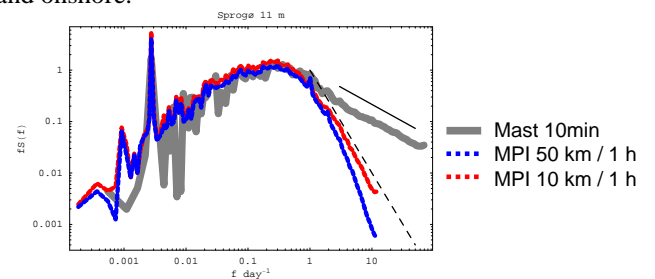
Figure 7. Measured (11m mast) PSD S_{[x,y]}(f) compared to climate model (MPI) PSD's S_{CM[x,y]}(f) for the Sprogø site.
