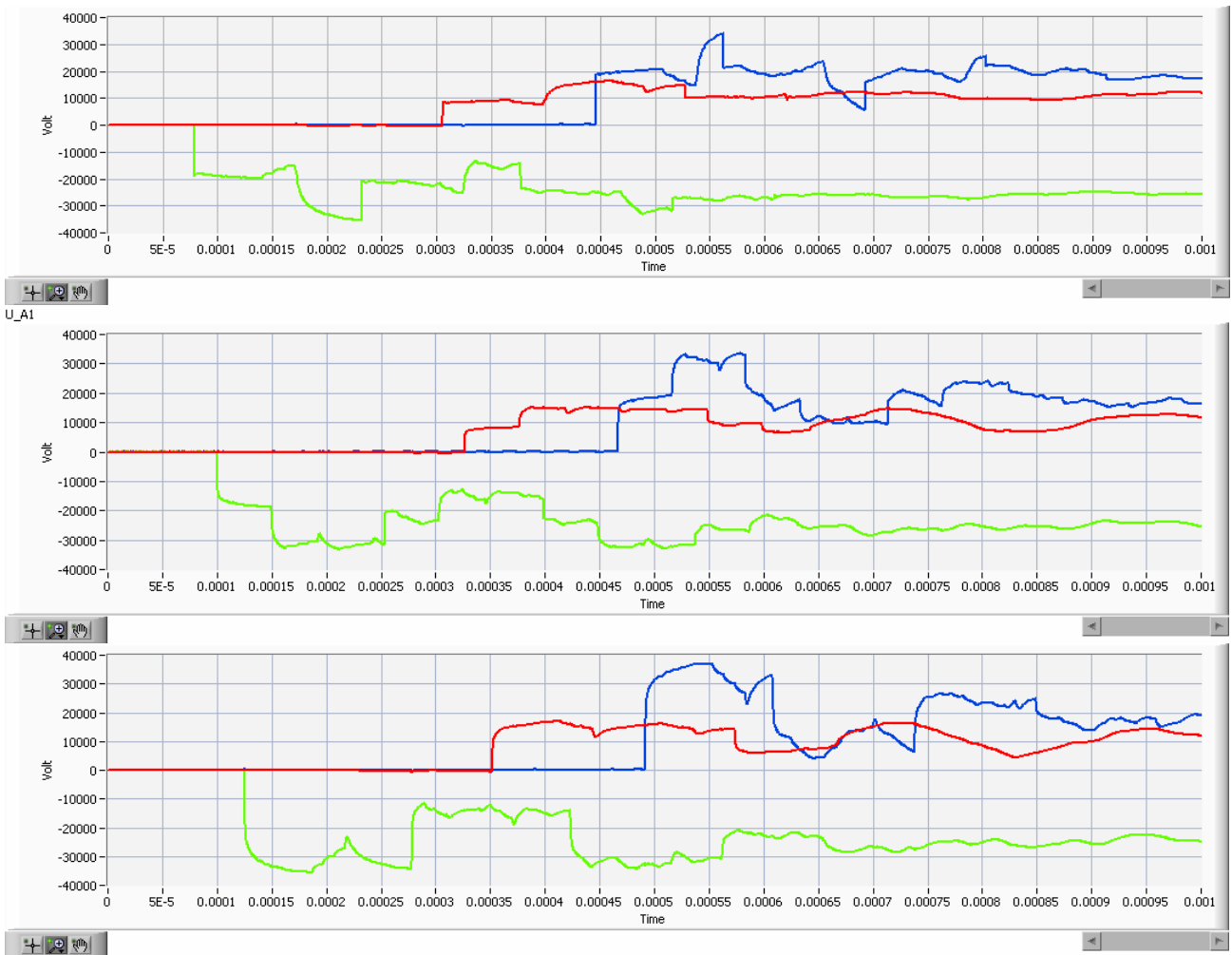
Figure 7 Voltage measurements at three locations during closing of the line breaker. Top: Transform platform, Middle: Turbine A01, Bottom: Turbine A09. Time: 50µs/div.
