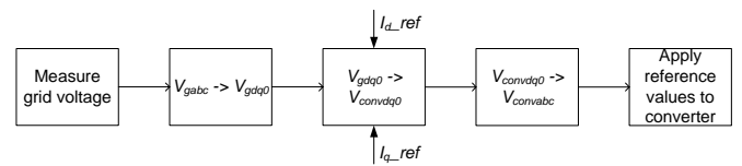
Figure 3 Schematic overview of current control.
