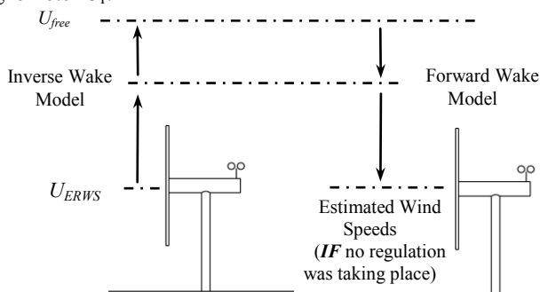
Figure 2-5: Overview of the Dynamic Plant Wake Model
