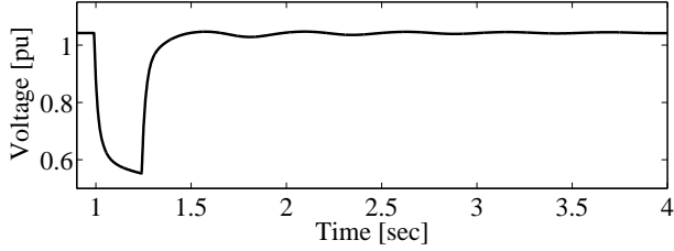
Fig. 3. Voltage profile
