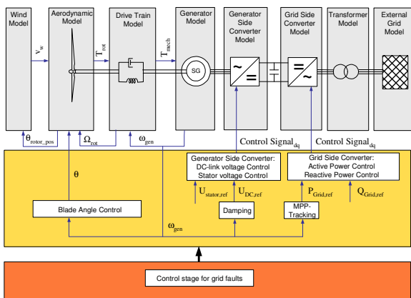
Figure 2: PMSG wind turbine dynamic simulation model and control strategy for normal operation and grid fault operation
