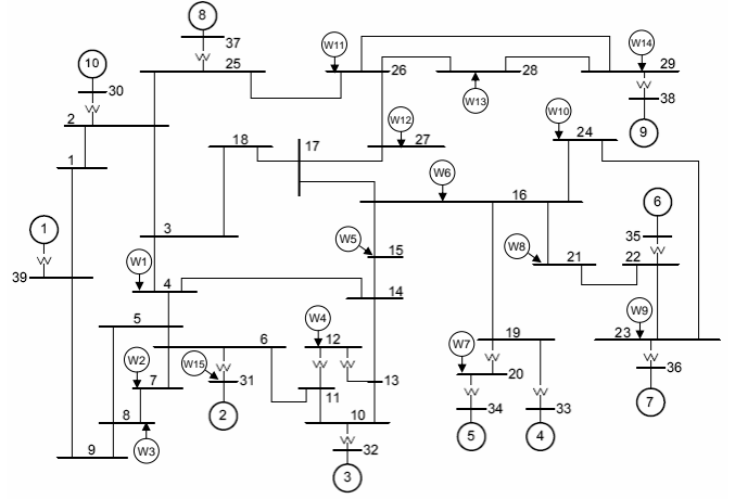
Fig. 1: IEEE New England Test System
