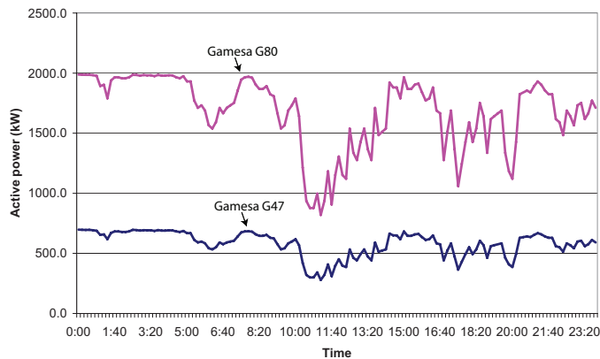
Fig. 3. Generated active power in January, 1
