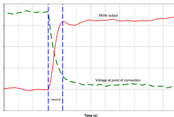
Figure 8 – Example of an upstream transformer tap test for determining voltage control performance
