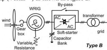
Figure 2. Partial variable speed wind turbine with variable rotor resistance.
