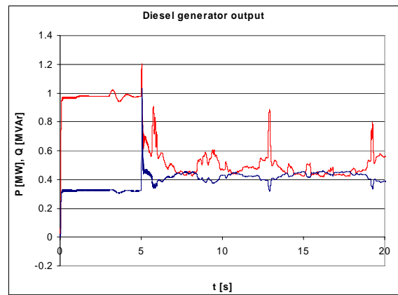
Figure 10. The output of the diesel generator.
