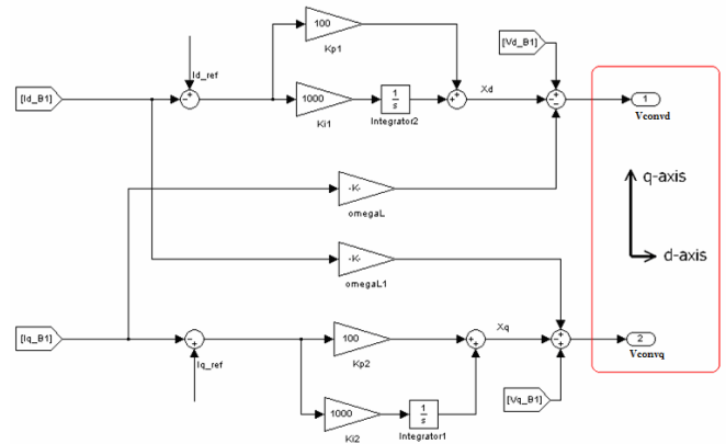
Figure 5 Current controller.
