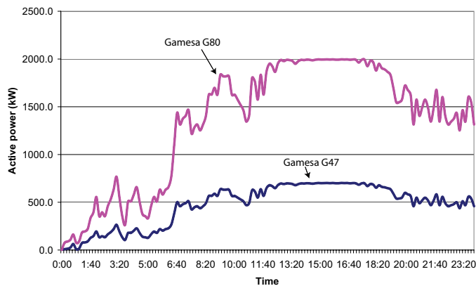
Fig. 4. Generated active power in July, 1
