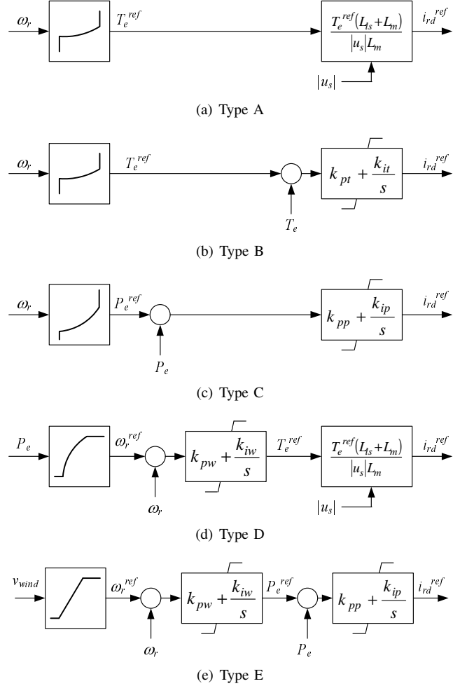
Fig. 4. Control schemes
