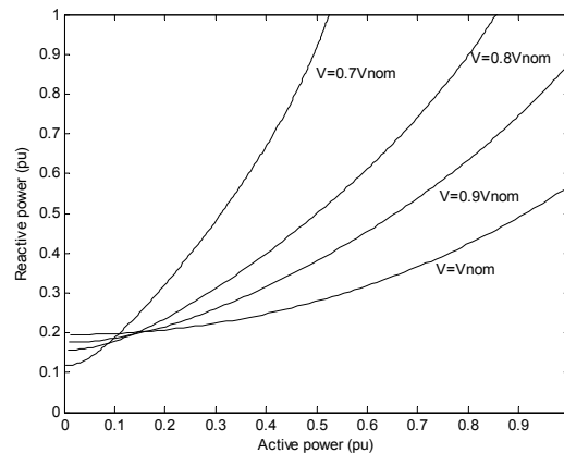
Figure 3. Reactive power consumed by an induction generator as a function of the generated active power for different voltage levels ( V_{nom} = nominal voltage).
