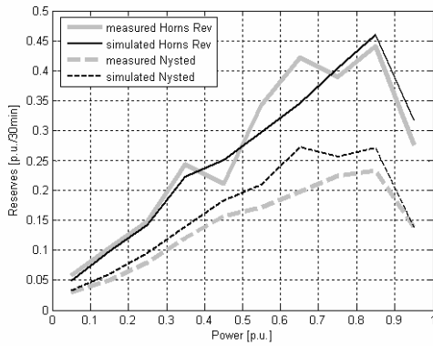
Figure 11. 1 % percentiles of 30 minutes reserve requirements in Horns Rev and Nysted wind farm
