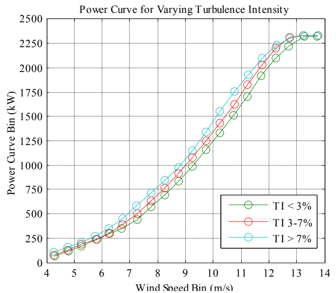
Figure 2-8: Example Turbulence Intensity Based Power Curves
