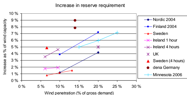
Figure 2. Results for the increase in reserve requirement due to wind power. German dena estimates are taking into account the day-ahead uncertainty (for up and down reserves separately). In Minnesota, day ahead uncertainty has been included in the forecast. For the others the effect of variations during the operating hour is considered. For UK, Ireland and Sweden the 4 hour-ahead uncertainty has been evaluated separately.
