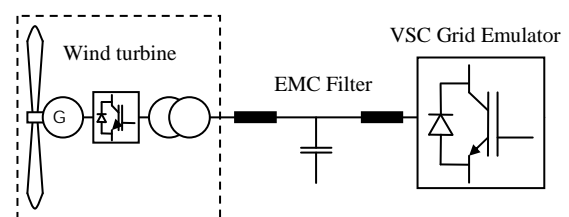
Fig. 2. Suitable test equipment: VSC grid emulator for code validation.
