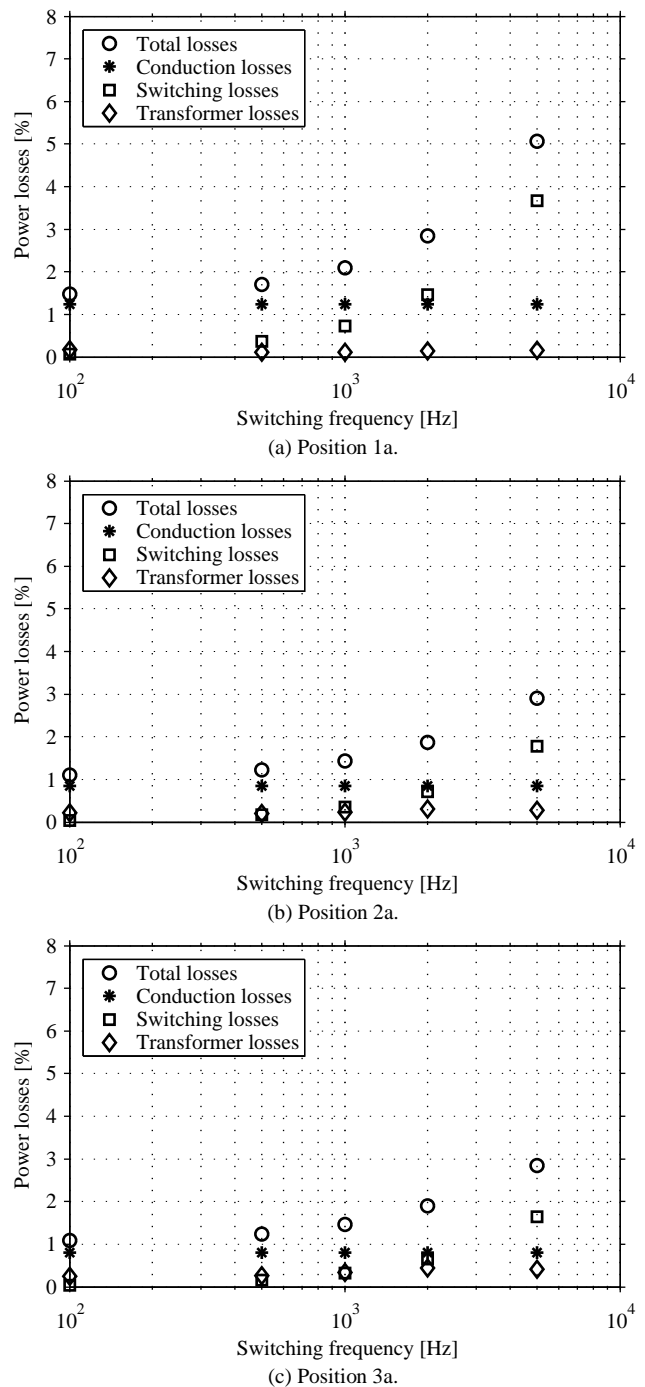
Figure 8. Loss distribution for IGBT module 2 using duty cycle control at the average wind speed 7.2m/s.
