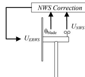
Figure 2-1: Determination of the Equivalent Rotor Wind Speed
