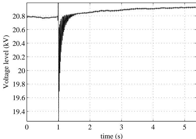
Fig. 6. Voltage level when cable is energized
