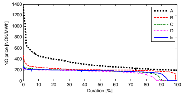
Figure 9. Duration curve for price in Norway for simulation cases A-E.
