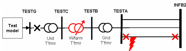
Figure 1. Test network BN1
