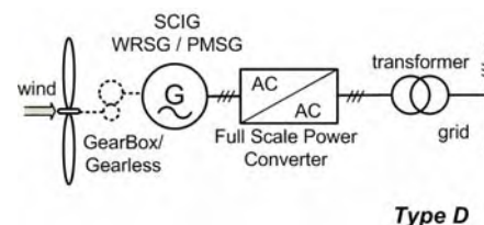
Figure 4. Variable speed wind turbine with full-scale power converter.
