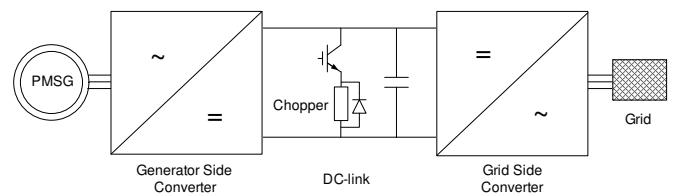
Figure 4: Chopper
