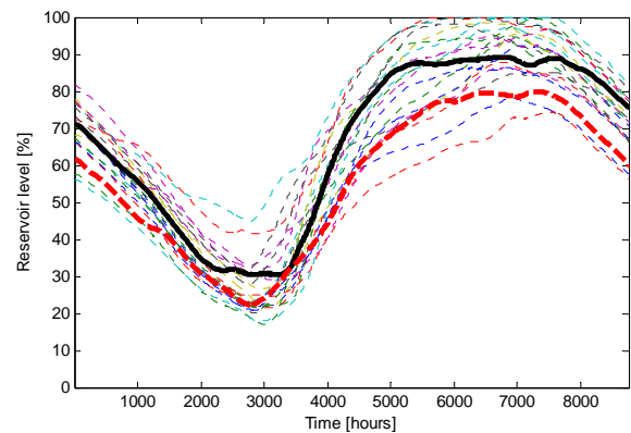
Figure 7. Simulated hydro reservoir level in Case B (15 TWh load increase and 35 TWh wind generation), using 21 consecutive years of inflow data. The solid thick line is the median level. The dotted thick line is the median level for the reference case.
