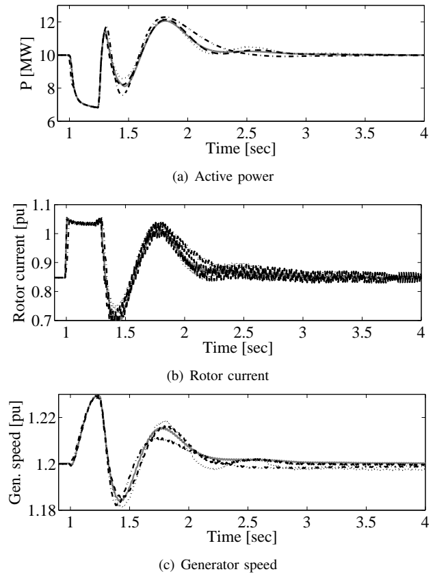
Fig. 7. Response of wind turbine with different controller schemes to grid fault: type A (solid), type C (dashed), type D (dotted) and type E (dash-dotted)
