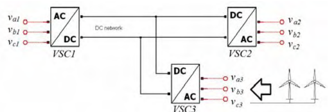
Figure 1 The proposed MT-VSC transmission system, all three converters are rated 300 MW.
