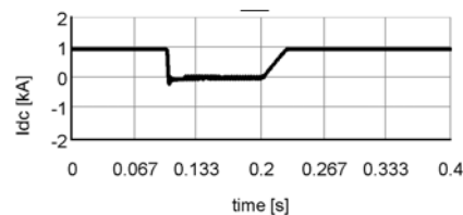
Figure 10 3-phase to ground fault at grid side of VSC2, power flow from VSC1 to VSC2.
