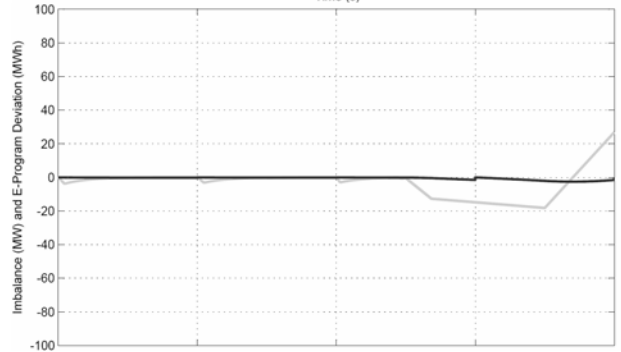
Fig. 7. Above: Scheduled (MW, grey line) and actual generation (MW, black line). Below: power imbalance (MW, grey line) and energy program deviation (MWh, black line). All for PRP 1 for simulation b).
