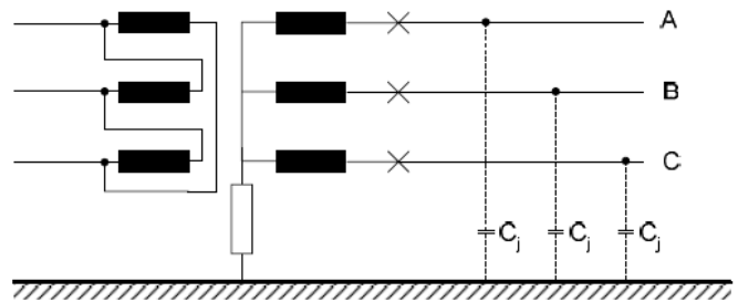
Figure 4. Resistance grounded system
