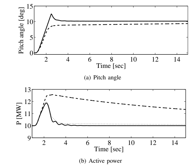
Fig. 10. Response of wind turbine to wind gust: with pitch compensation (solid), no pitch compensation (dashed) and no pitch compensation with adjusted controller gain (dotted)
