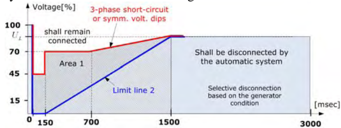
Figure 16. Voltage limits for disconnection of wind turbines in the case of faults in the German transmission networks [26].
